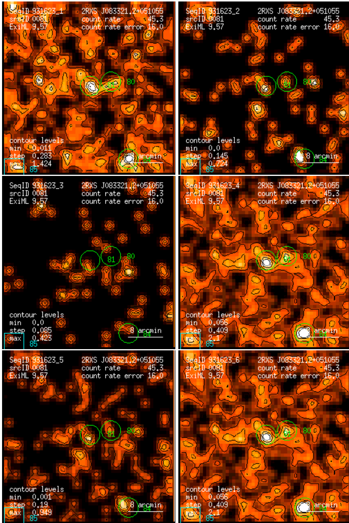
Figure 81: RASS 931623: detection 0081: band rate images, Gaussian filter: (1) PSPC channels 11 – 41, (2) 52 – 90, (3) 91 – 201, (4) 11 – 235, (5) 52 – 201, (6) 11 – 201. Broad band rates in counts/ks. Band rate contour levels in counts/ks/arcmin 2 .
