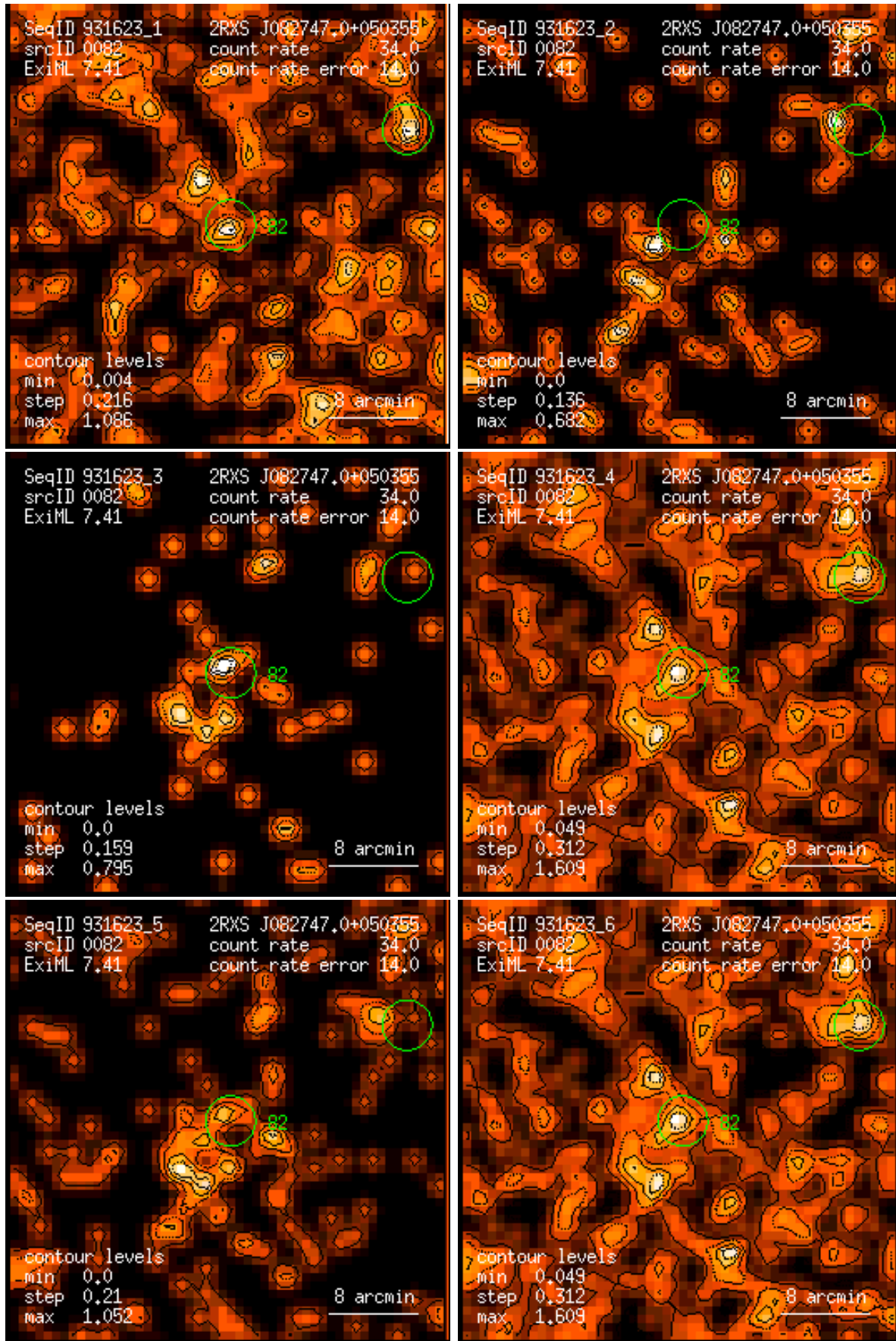
Figure 82: RASS 931623: detection 0082: band rate images, Gaussian filter: (1) PSPC channels 11 – 41, (2) 52 – 90, (3) 91 – 201, (4) 11 – 235, (5) 52 – 201, (6) 11 – 201. Broad band rates in counts/ks. Band rate contour levels in counts/ks/arcmin 2 .
