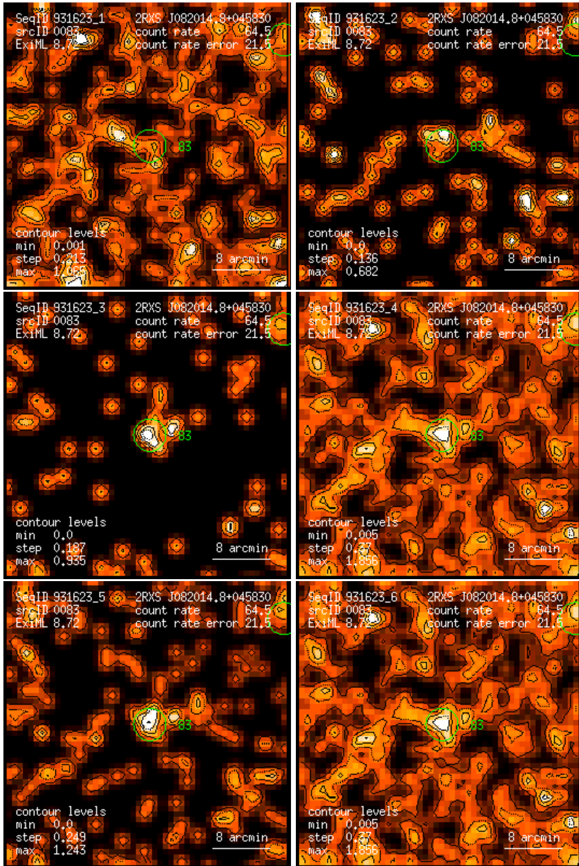
Figure 83: RASS 931623: detection 0083: band rate images, Gaussian filter: (1) PSPC channels 11 – 41, (2) 52 – 90, (3) 91 – 201, (4) 11 – 235, (5) 52 – 201, (6) 11 – 201. Broad band rates in counts/ks. Band rate contour levels in counts/ks/arcmin 2 .
