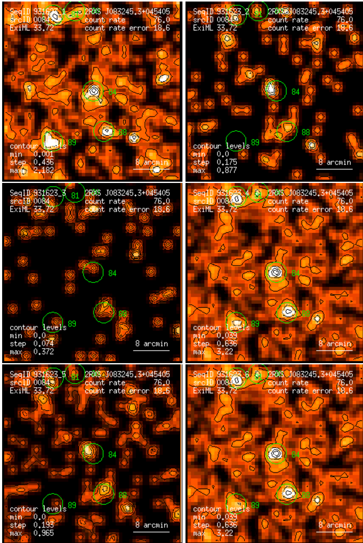
Figure 84: RASS 931623: detection 0084: band rate images, Gaussian filter: (1) PSPC channels 11 – 41, (2) 52 – 90, (3) 91 – 201, (4) 11 – 235, (5) 52 – 201, (6) 11 – 201. Broad band rates in counts/ks. Band rate contour levels in counts/ks/arcmin 2 .
