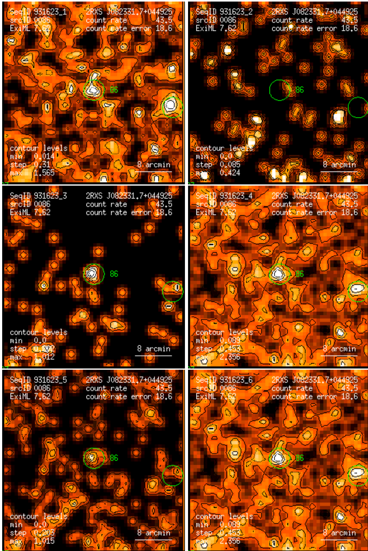
Figure 86: RASS 931623: detection 0086: band rate images, Gaussian filter: (1) PSPC channels 11 – 41, (2) 52 – 90, (3) 91 – 201, (4) 11 – 235, (5) 52 – 201, (6) 11 – 201. Broad band rates in counts/ks. Band rate contour levels in counts/ks/arcmin 2 .
