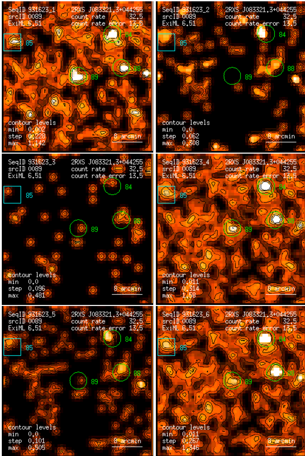
Figure 89: RASS 931623: detection 0089: band rate images, Gaussian filter: (1) PSPC channels 11 – 41, (2) 52 – 90, (3) 91 – 201, (4) 11 – 235, (5) 52 – 201, (6) 11 – 201. Broad band rates in counts/ks. Band rate contour levels in counts/ks/arcmin 2 .
