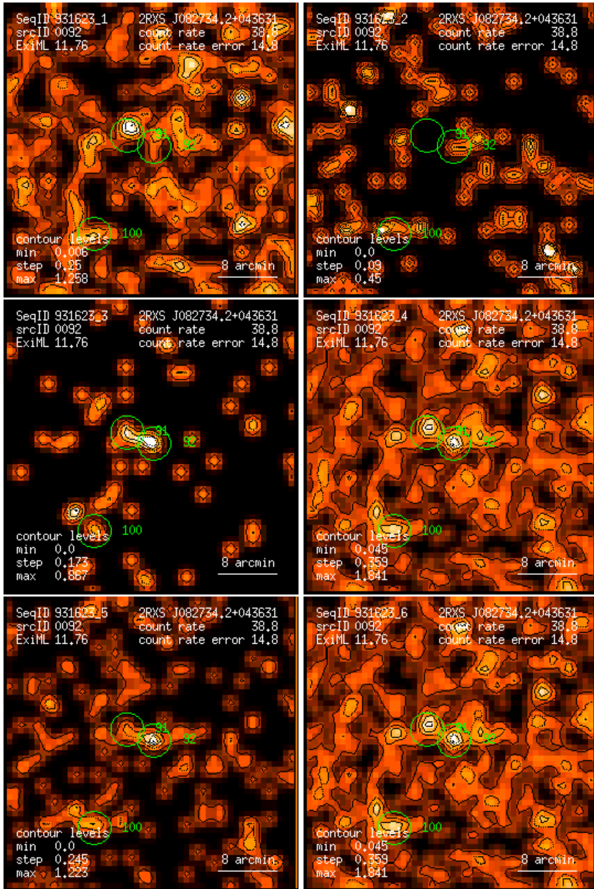
Figure 92: RASS 931623: detection 0092: band rate images, Gaussian filter: (1) PSPC channels 11 – 41, (2) 52 – 90, (3) 91 – 201, (4) 11 – 235, (5) 52 – 201, (6) 11 – 201. Broad band rates in counts/ks. Band rate contour levels in counts/ks/arcmin 2 .
