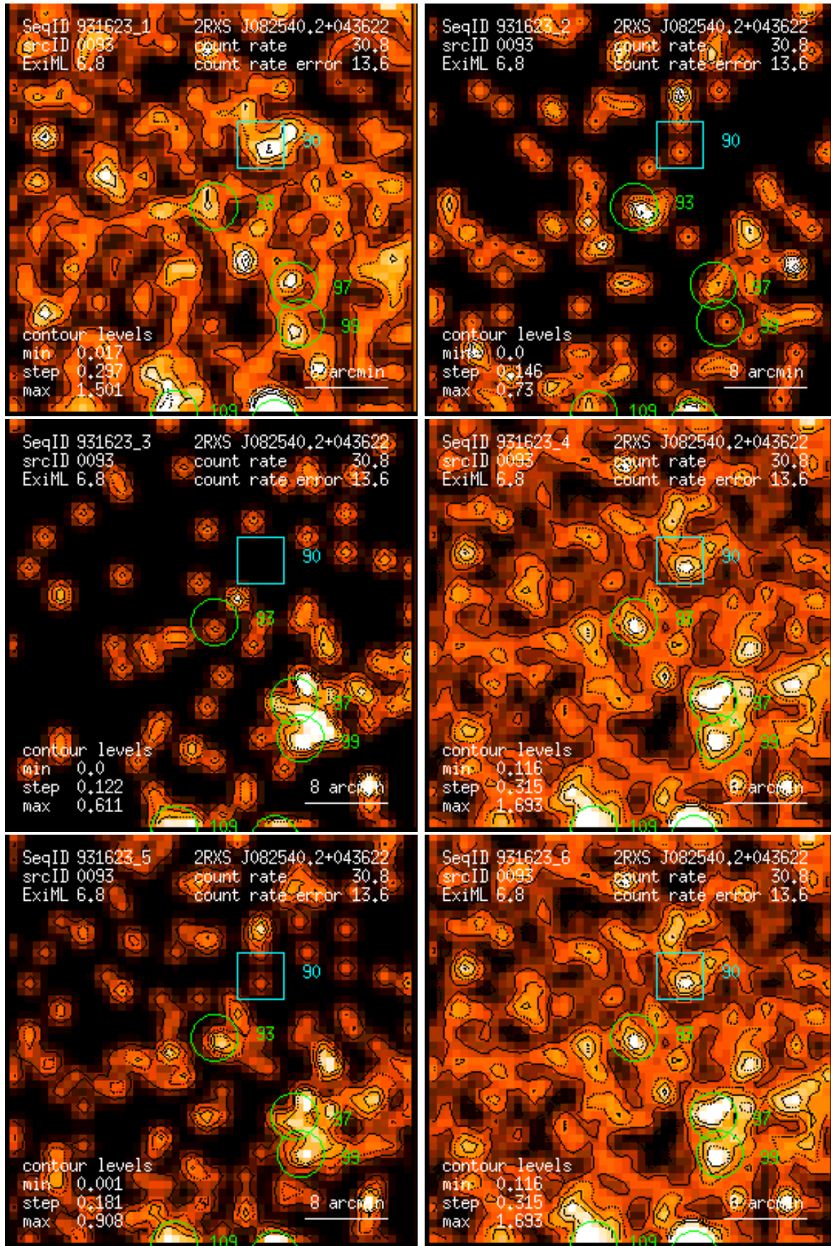
Figure 93: RASS 931623: detection 0093: band rate images, Gaussian filter: (1) PSPC channels 11 – 41, (2) 52 – 90, (3) 91 – 201, (4) 11 – 235, (5) 52 – 201, (6) 11 – 201. Broad band rates in counts/ks. Band rate contour levels in counts/ks/arcmin 2 .
