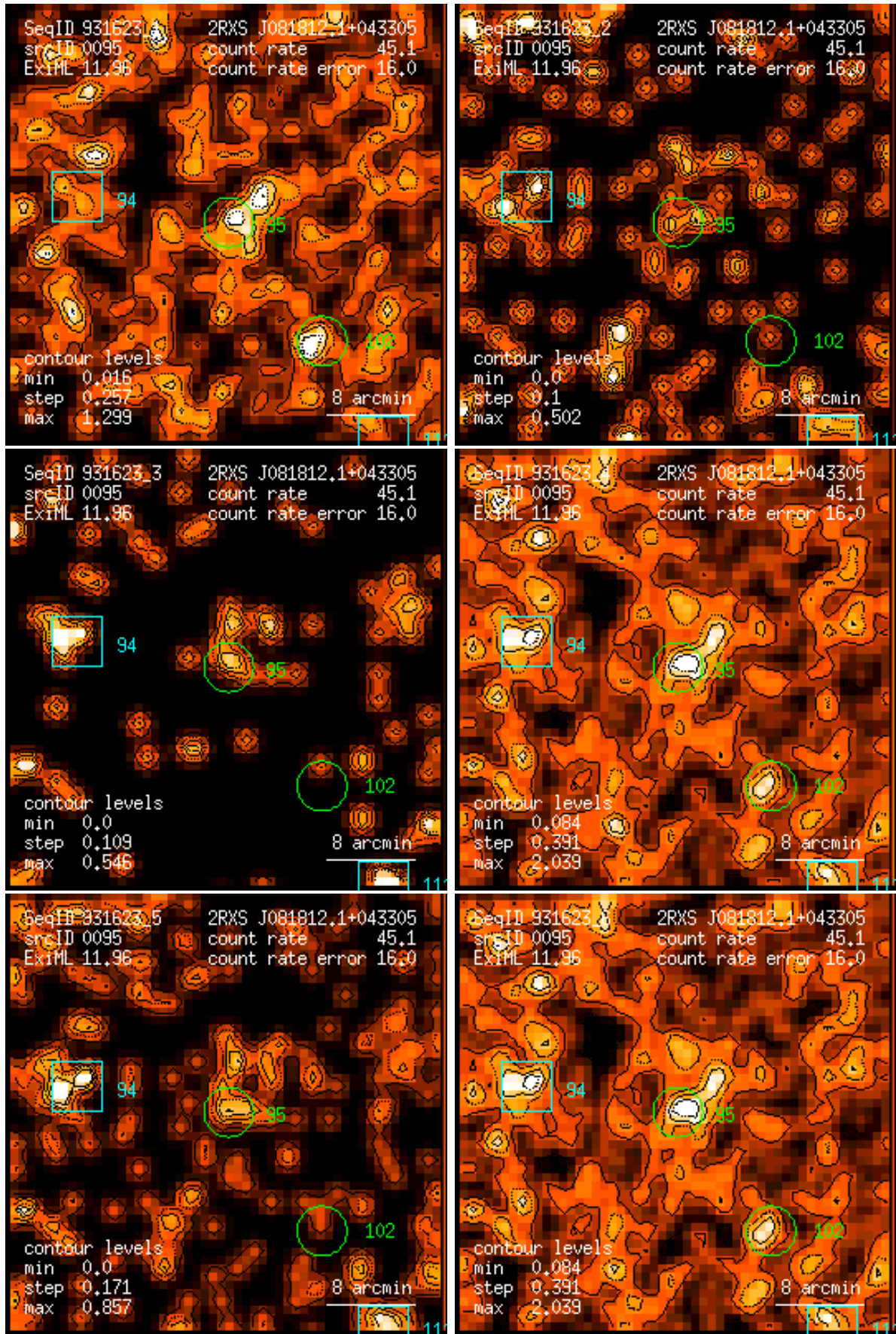
Figure 95: RASS 931623: detection 0095: band rate images, Gaussian filter: (1) PSPC channels 11 – 41, (2) 52 – 90, (3) 91 – 201, (4) 11 – 235, (5) 52 – 201, (6) 11 – 201. Broad band rates in counts/ks. Band rate contour levels in counts/ks/arcmin 2 .
