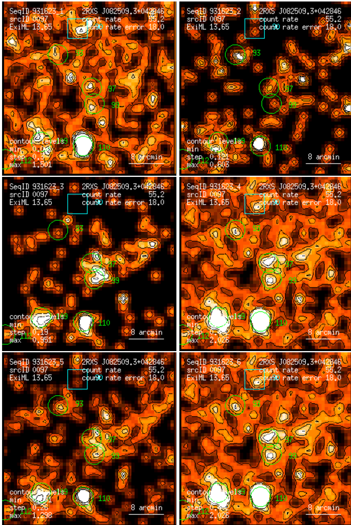
Figure 97: RASS 931623: detection 0097: band rate images, Gaussian filter: (1) PSPC channels 11 – 41, (2) 52 – 90, (3) 91 – 201, (4) 11 – 235, (5) 52 – 201, (6) 11 – 201. Broad band rates in counts/ks. Band rate contour levels in counts/ks/arcmin 2 .
