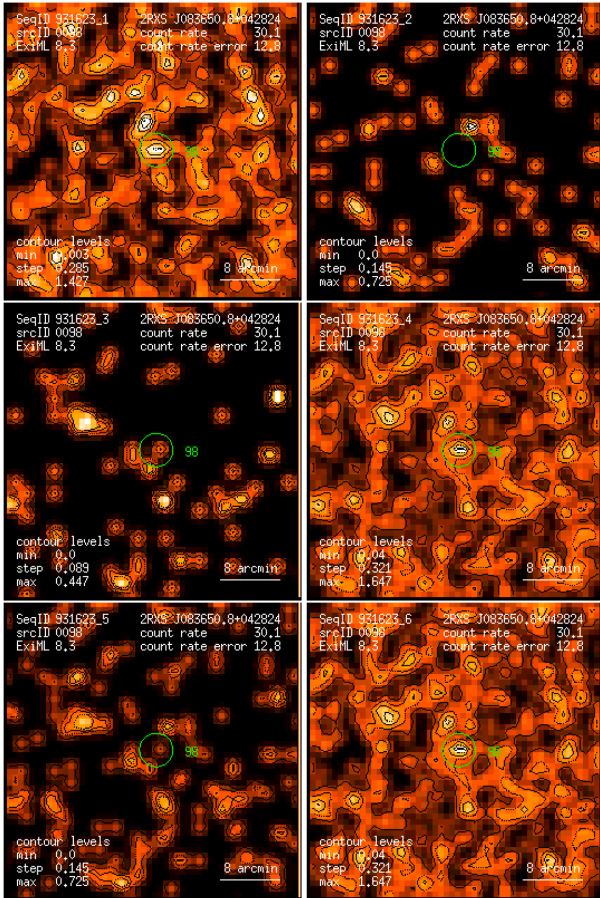
Figure 98: RASS 931623: detection 0098: band rate images, Gaussian filter: (1) PSPC channels 11 – 41, (2) 52 – 90, (3) 91 – 201, (4) 11 – 235, (5) 52 – 201, (6) 11 – 201. Broad band rates in counts/ks. Band rate contour levels in counts/ks/arcmin 2 .
