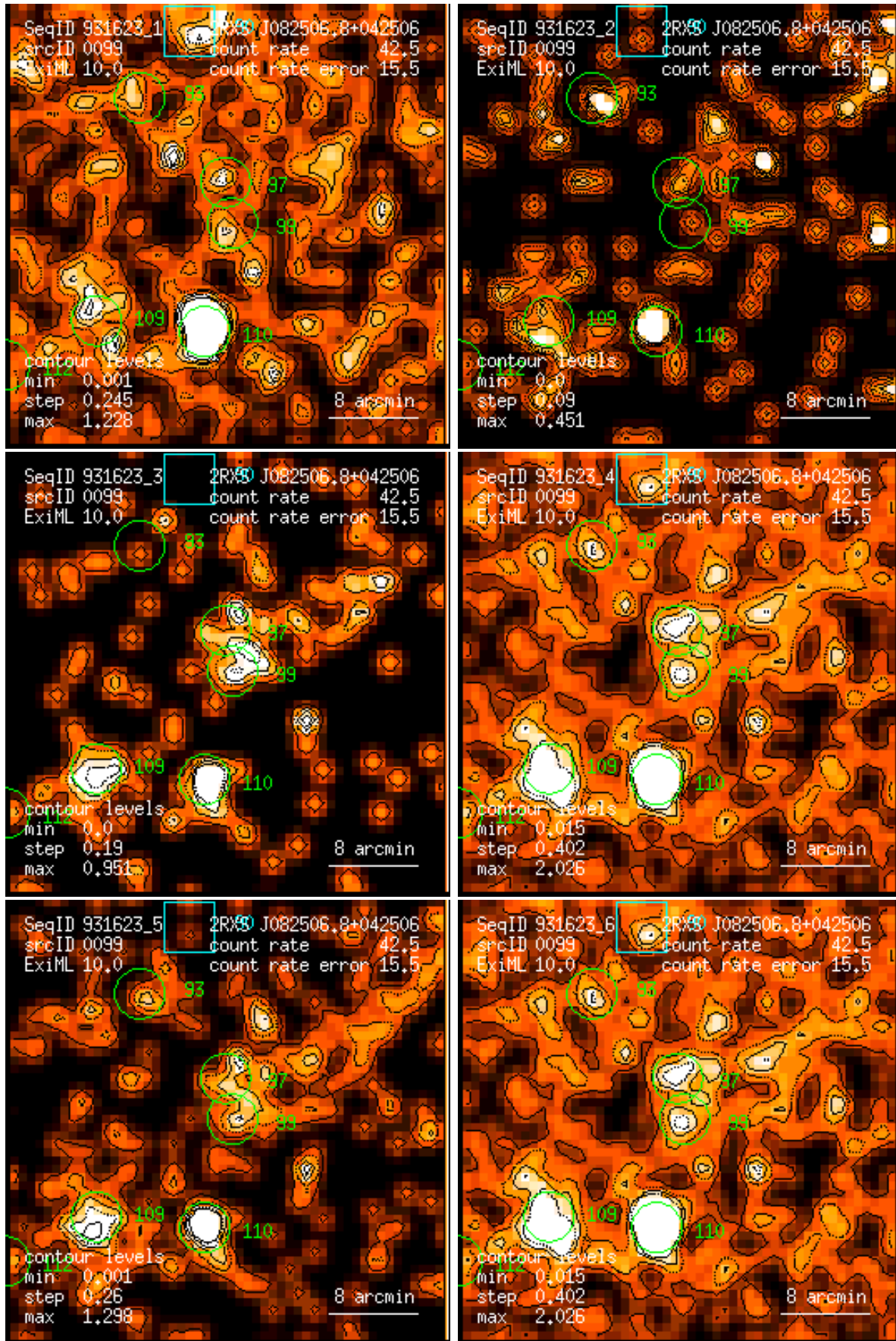
Figure 99: RASS 931623: detection 0099: band rate images, Gaussian filter: (1) PSPC channels 11 – 41, (2) 52 – 90, (3) 91 – 201, (4) 11 – 235, (5) 52 – 201, (6) 11 – 201. Broad band rates in counts/ks. Band rate contour levels in counts/ks/arcmin 2 .
