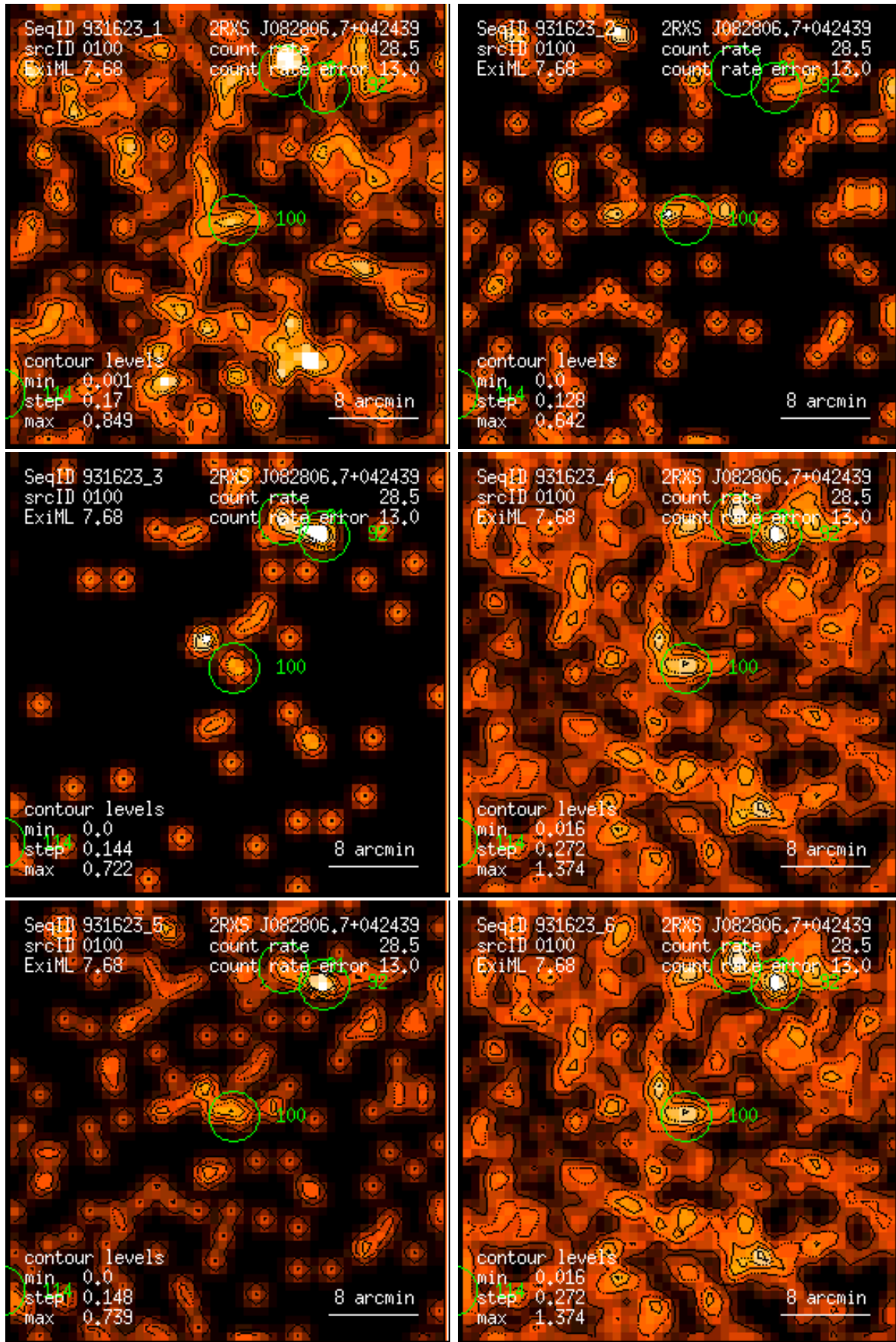
Figure 100: RASS 931623: detection 0100: band rate images, Gaussian filter: (1) PSPC channels 11 – 41, (2) 52 – 90, (3) 91 – 201, (4) 11 – 235, (5) 52 – 201, (6) 11 – 201. Broad band rates in counts/ks. Band rate contour levels in counts/ks/arcmin 2 .
