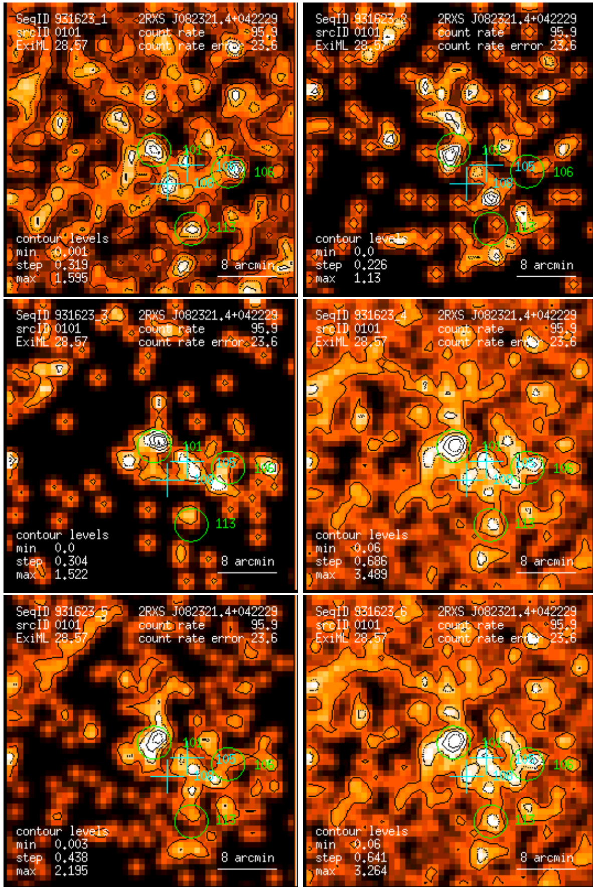
Figure 101: RASS 931623: detection 0101: band rate images, Gaussian filter: (1) PSPC channels 11 – 41, (2) 52 – 90, (3) 91 – 201, (4) 11 – 235, (5) 52 – 201, (6) 11 – 201. Broad band rates in counts/ks. Band rate contour levels in counts/ks/arcmin 2 .
