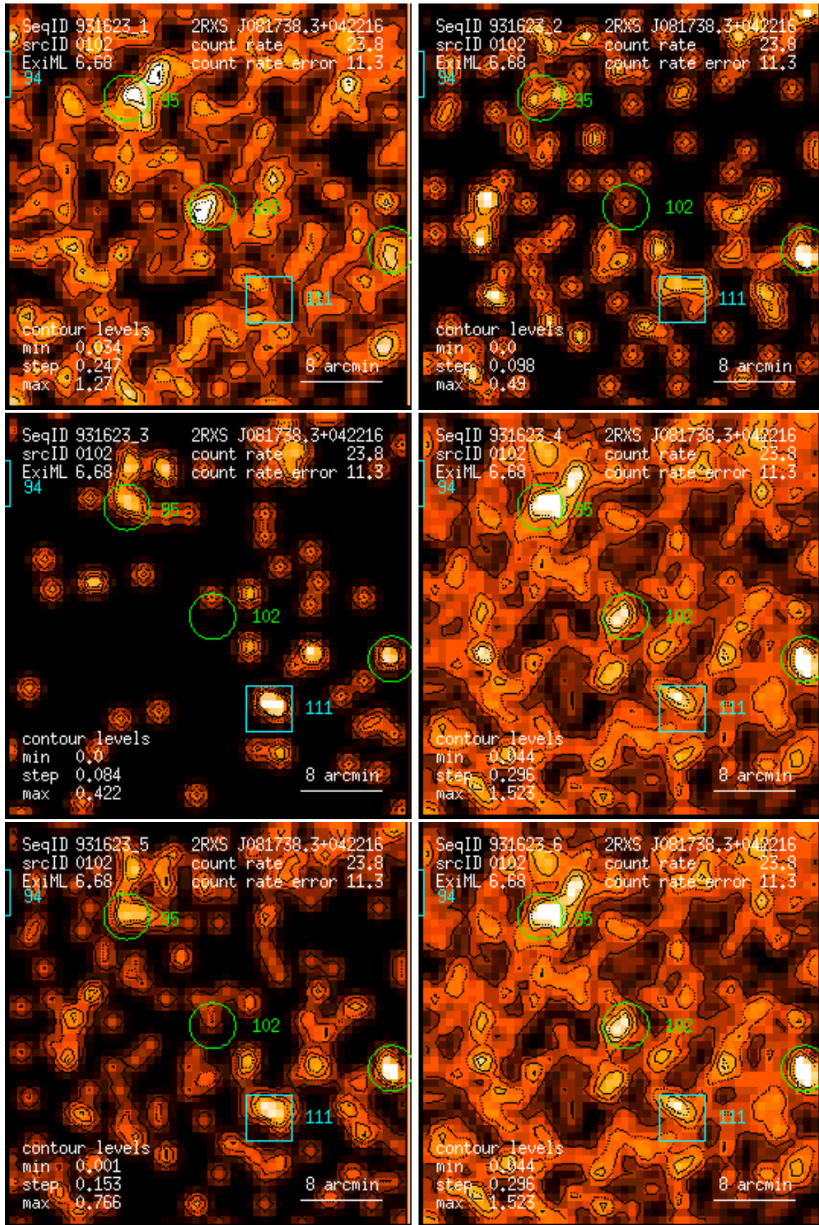
Figure 102: RASS 931623: detection 0102: band rate images, Gaussian filter: (1) PSPC channels 11 – 41, (2) 52 – 90, (3) 91 – 201, (4) 11 – 235, (5) 52 – 201, (6) 11 – 201. Broad band rates in counts/ks. Band rate contour levels in counts/ks/arcmin 2 .
