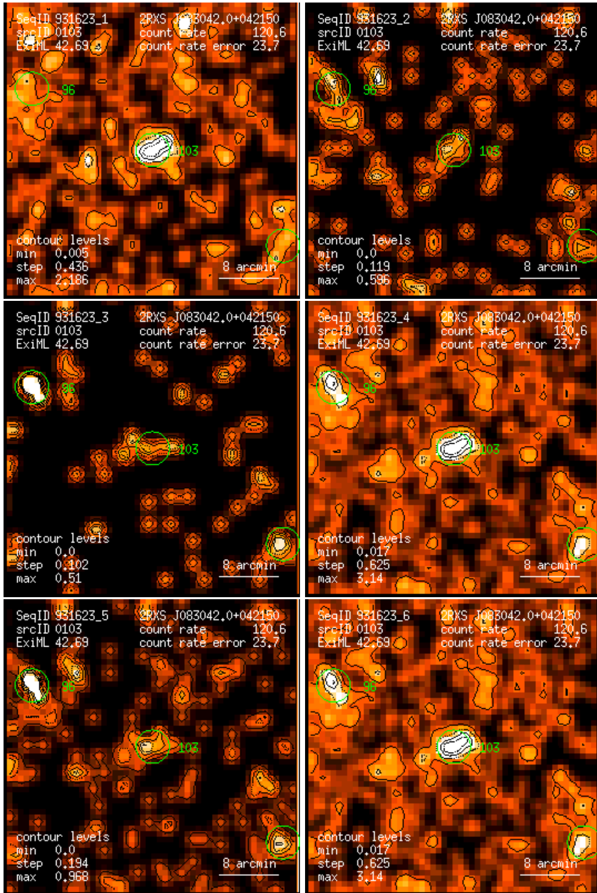
Figure 103: RASS 931623: detection 0103: band rate images, Gaussian filter: (1) PSPC channels 11 – 41, (2) 52 – 90, (3) 91 – 201, (4) 11 – 235, (5) 52 – 201, (6) 11 – 201. Broad band rates in counts/ks. Band rate contour levels in counts/ks/arcmin 2 .
