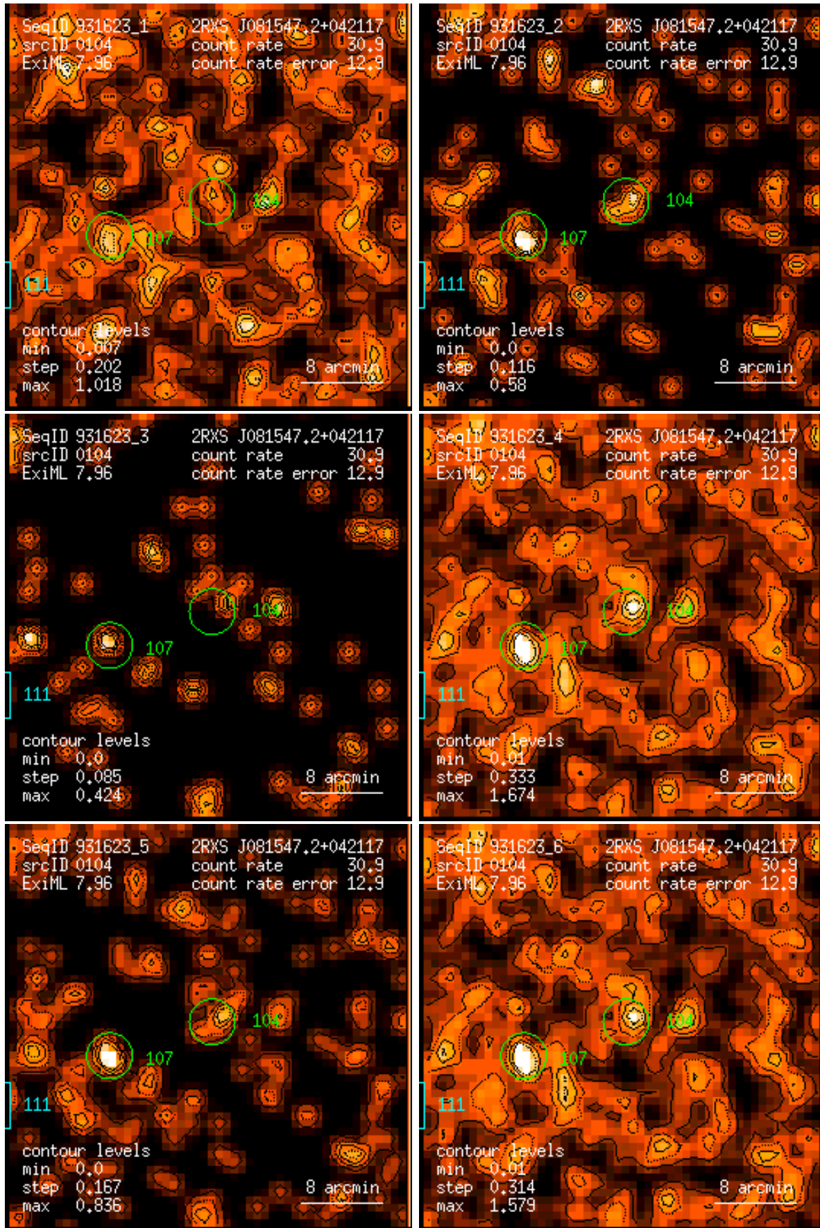
Figure 104: RASS 931623: detection 0104: band rate images, Gaussian filter: (1) PSPC channels 11 – 41, (2) 52 – 90, (3) 91 – 201, (4) 11 – 235, (5) 52 – 201, (6) 11 – 201. Broad band rates in counts/ks. Band rate contour levels in counts/ks/arcmin 2 .
