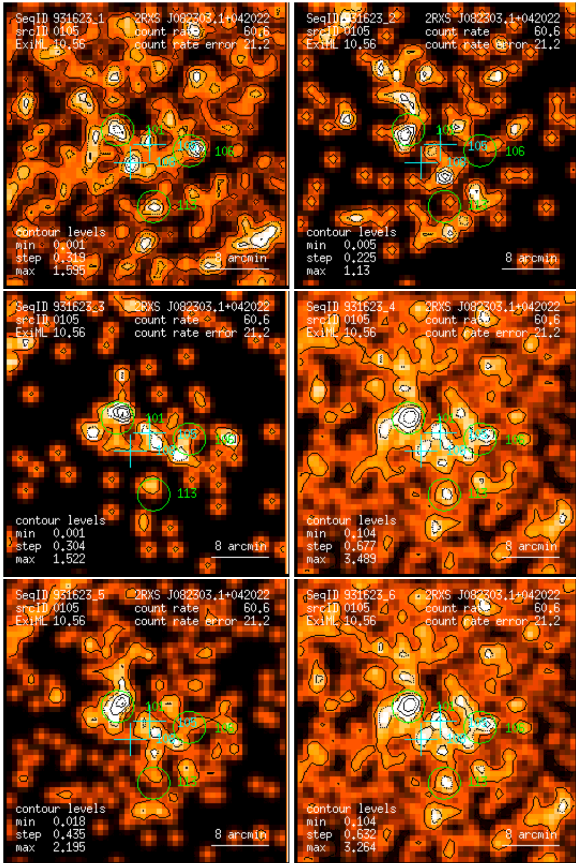
Figure 105: RASS 931623: detection 0105: band rate images, Gaussian filter: (1) PSPC channels 11 – 41, (2) 52 – 90, (3) 91 – 201, (4) 11 – 235, (5) 52 – 201, (6) 11 – 201. Broad band rates in counts/ks. Band rate contour levels in counts/ks/arcmin 2 .
