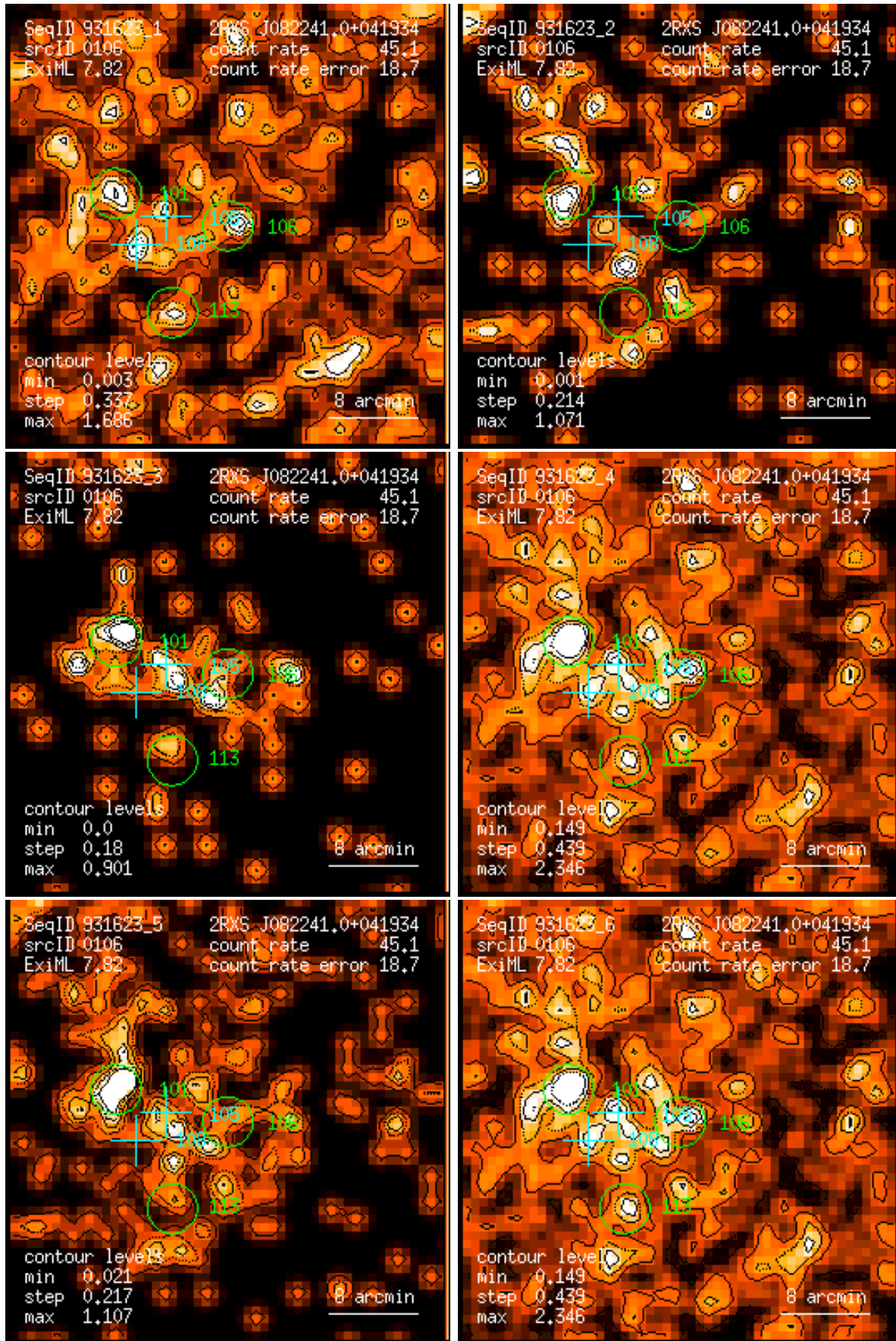
Figure 106: RASS 931623: detection 0106: band rate images, Gaussian filter: (1) PSPC channels 11 – 41, (2) 52 – 90, (3) 91 – 201, (4) 11 – 235, (5) 52 – 201, (6) 11 – 201. Broad band rates in counts/ks. Band rate contour levels in counts/ks/arcmin 2 .
