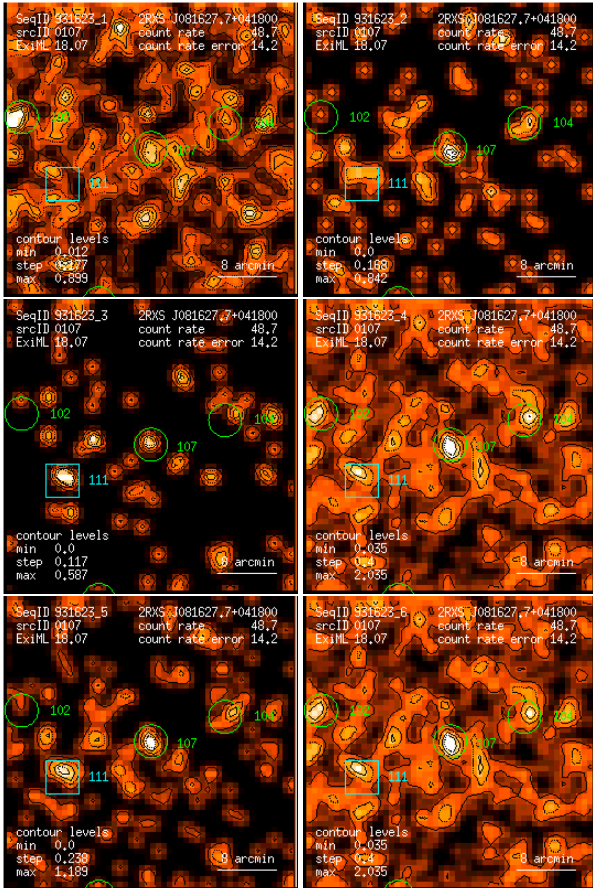
Figure 107: RASS 931623: detection 0107: band rate images, Gaussian filter: (1) PSPC channels 11 – 41, (2) 52 – 90, (3) 91 – 201, (4) 11 – 235, (5) 52 – 201, (6) 11 – 201. Broad band rates in counts/ks. Band rate contour levels in counts/ks/arcmin 2 .
