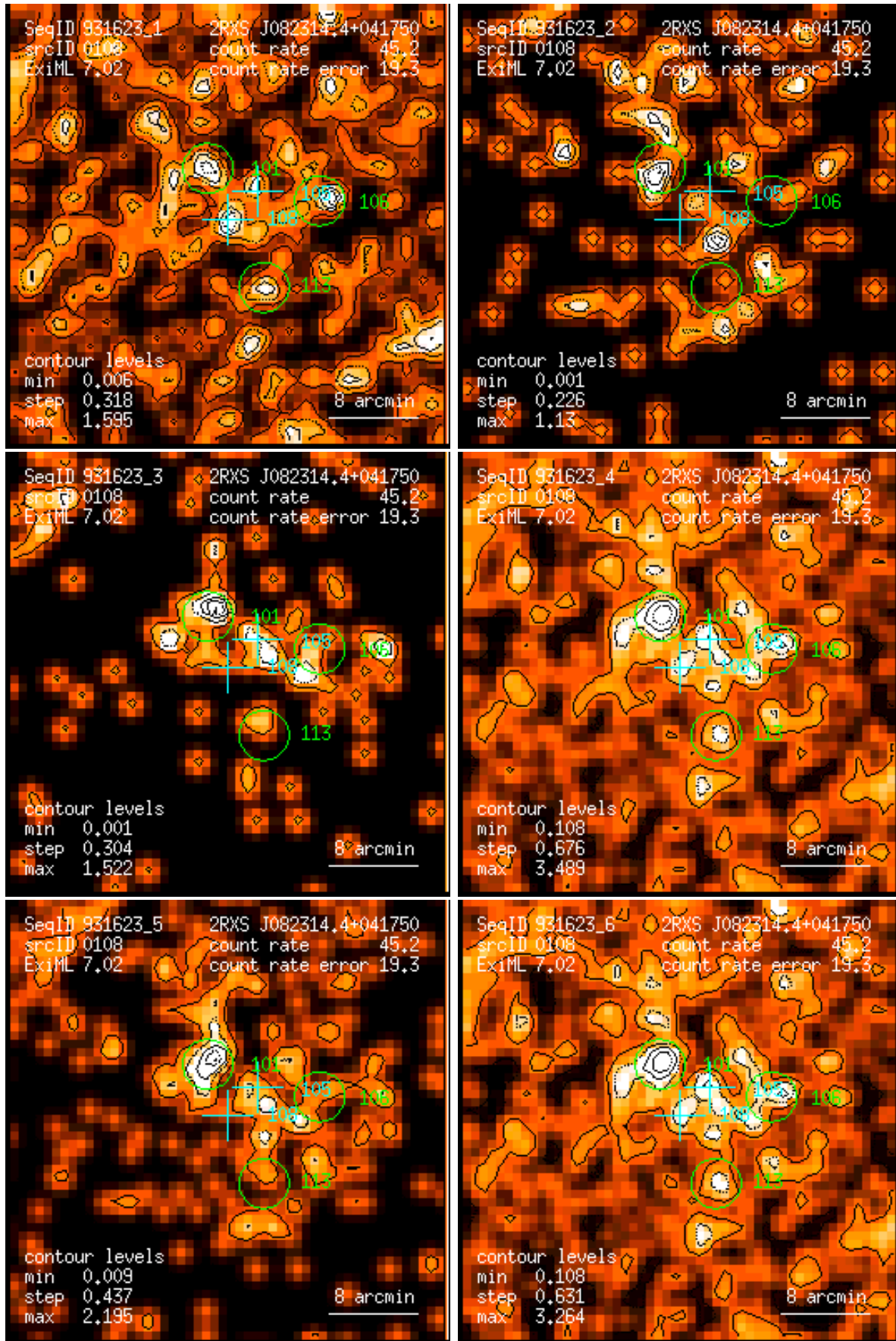
Figure 108: RASS 931623: detection 0108: band rate images, Gaussian filter: (1) PSPC channels 11 – 41, (2) 52 – 90, (3) 91 – 201, (4) 11 – 235, (5) 52 – 201, (6) 11 – 201. Broad band rates in counts/ks. Band rate contour levels in counts/ks/arcmin 2 .
