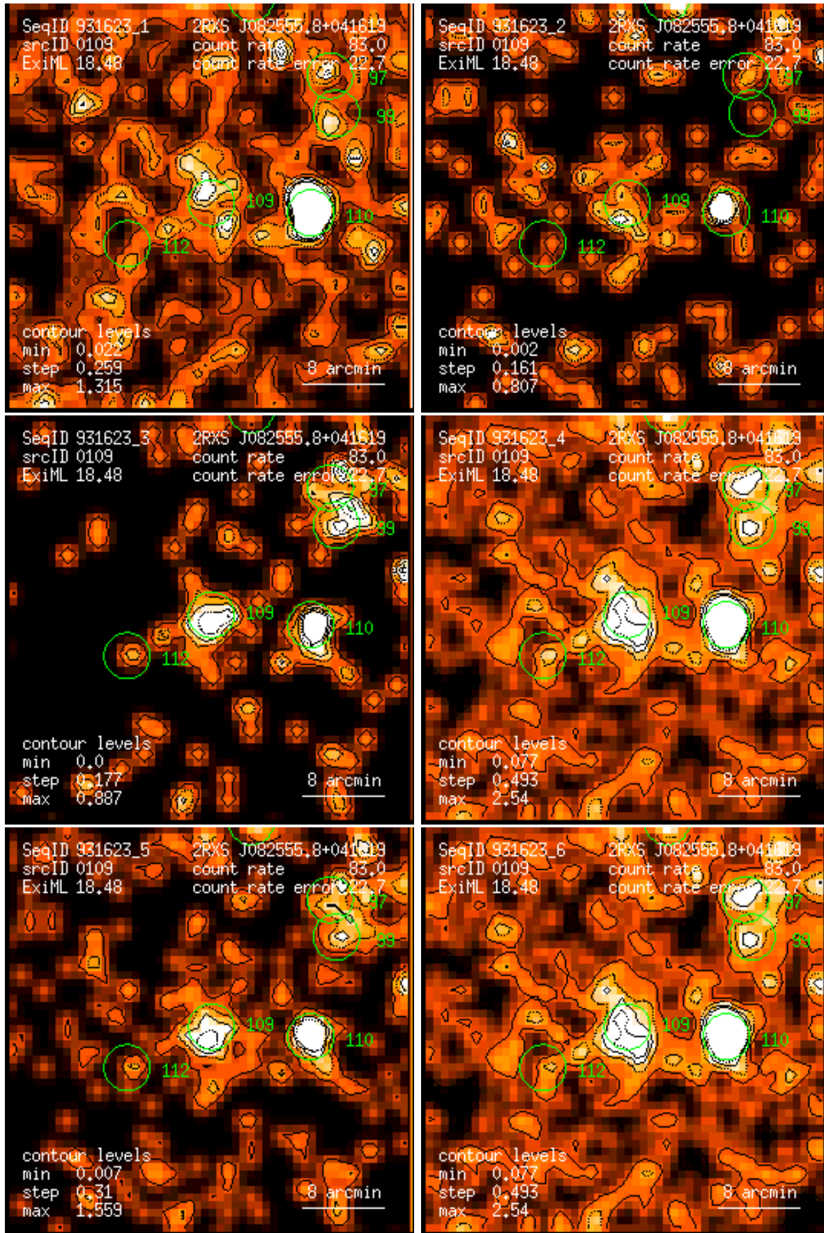
Figure 109: RASS 931623: detection 0109: band rate images, Gaussian filter: (1) PSPC channels 11 – 41, (2) 52 – 90, (3) 91 – 201, (4) 11 – 235, (5) 52 – 201, (6) 11 – 201. Broad band rates in counts/ks. Band rate contour levels in counts/ks/arcmin 2 .
