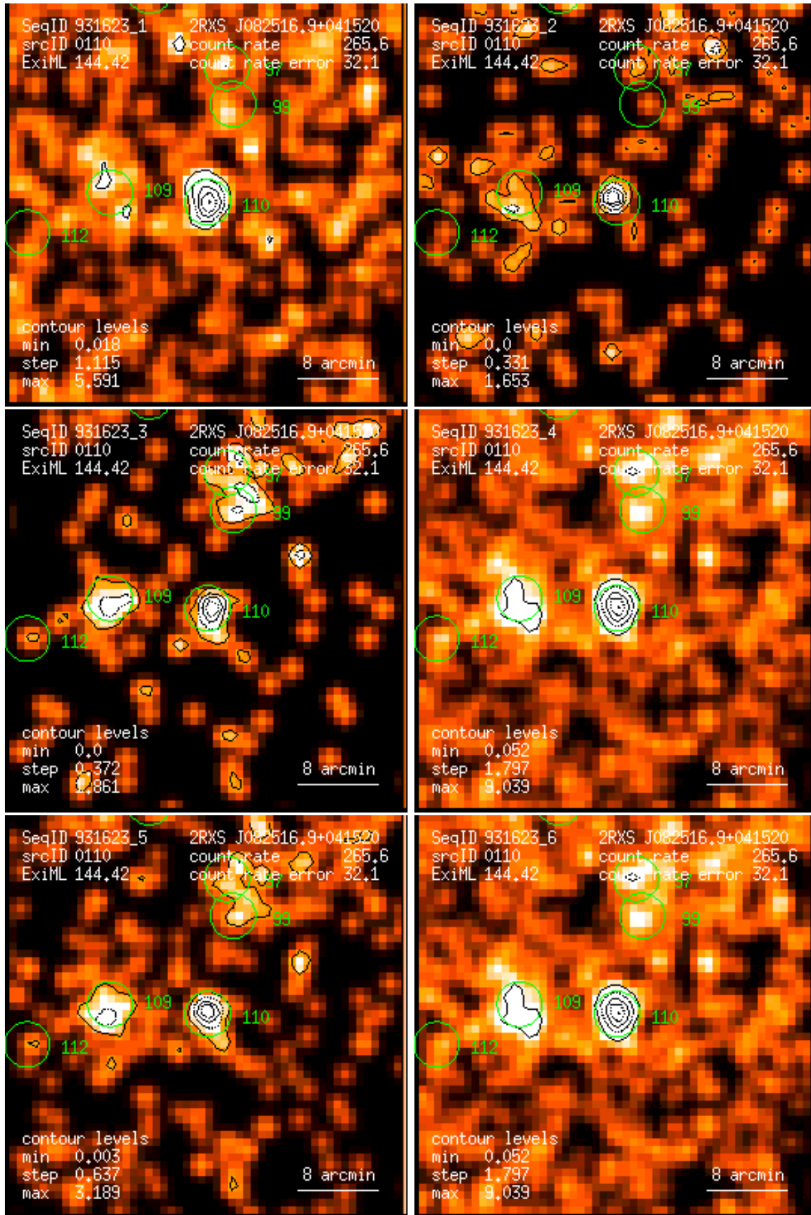
Figure 110: RASS 931623: detection 0110: band rate images, Gaussian filter: (1) PSPC channels 11 – 41, (2) 52 – 90, (3) 91 – 201, (4) 11 – 235, (5) 52 – 201, (6) 11 – 201. Broad band rates in counts/ks. Band rate contour levels in counts/ks/arcmin 2 .
