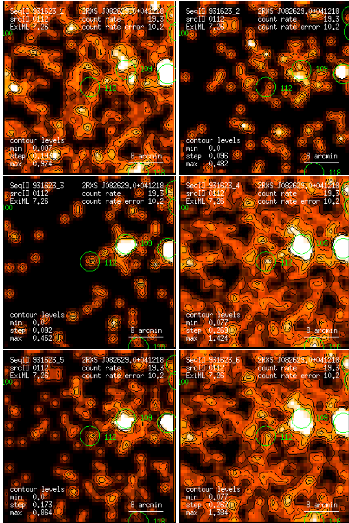
Figure 112: RASS 931623: detection 0112: band rate images, Gaussian filter: (1) PSPC channels 11 – 41, (2) 52 – 90, (3) 91 – 201, (4) 11 – 235, (5) 52 – 201, (6) 11 – 201. Broad band rates in counts/ks. Band rate contour levels in counts/ks/arcmin 2 .
