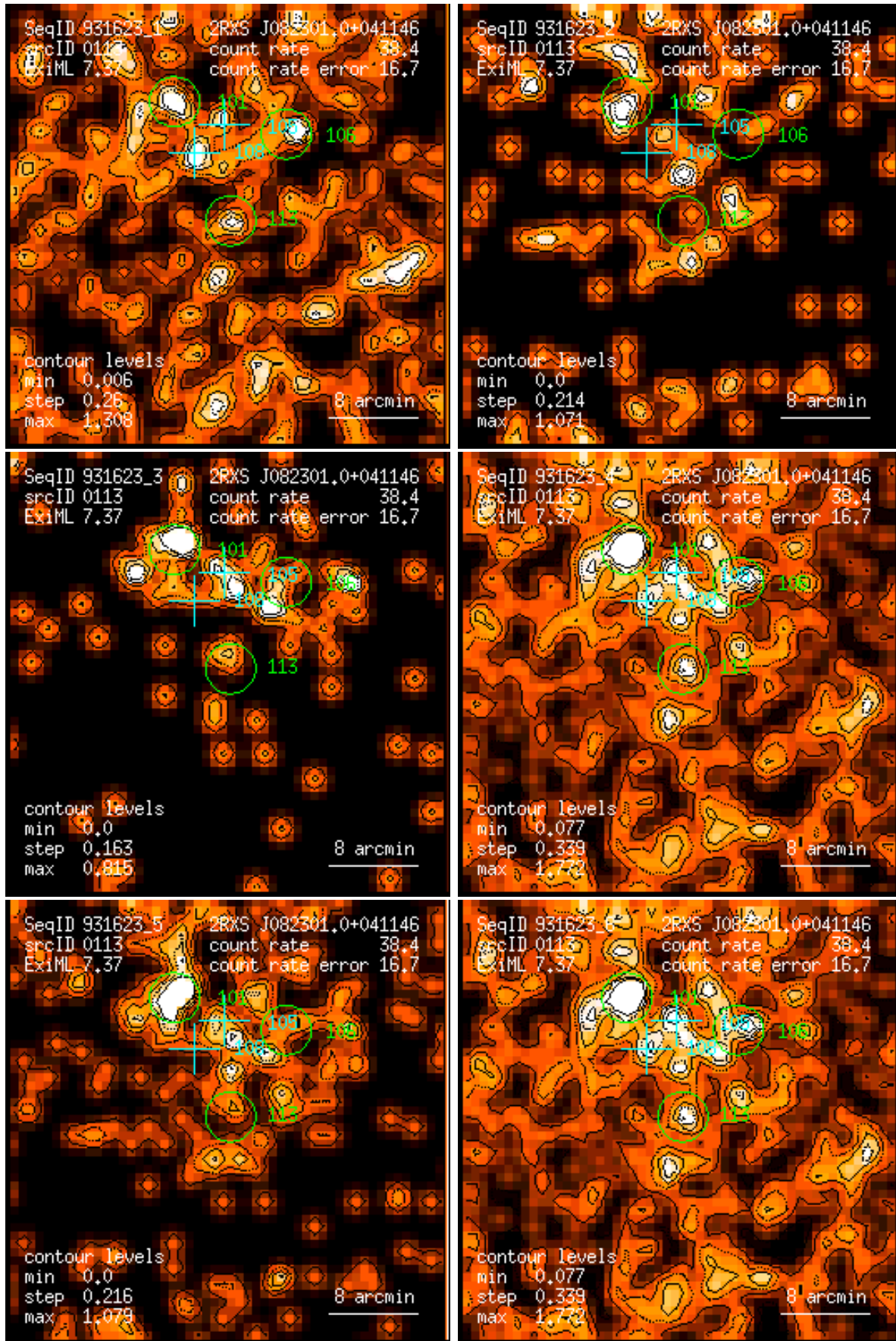
Figure 113: RASS 931623: detection 0113: band rate images, Gaussian filter: (1) PSPC channels 11 – 41, (2) 52 – 90, (3) 91 – 201, (4) 11 – 235, (5) 52 – 201, (6) 11 – 201. Broad band rates in counts/ks. Band rate contour levels in counts/ks/arcmin 2 .
