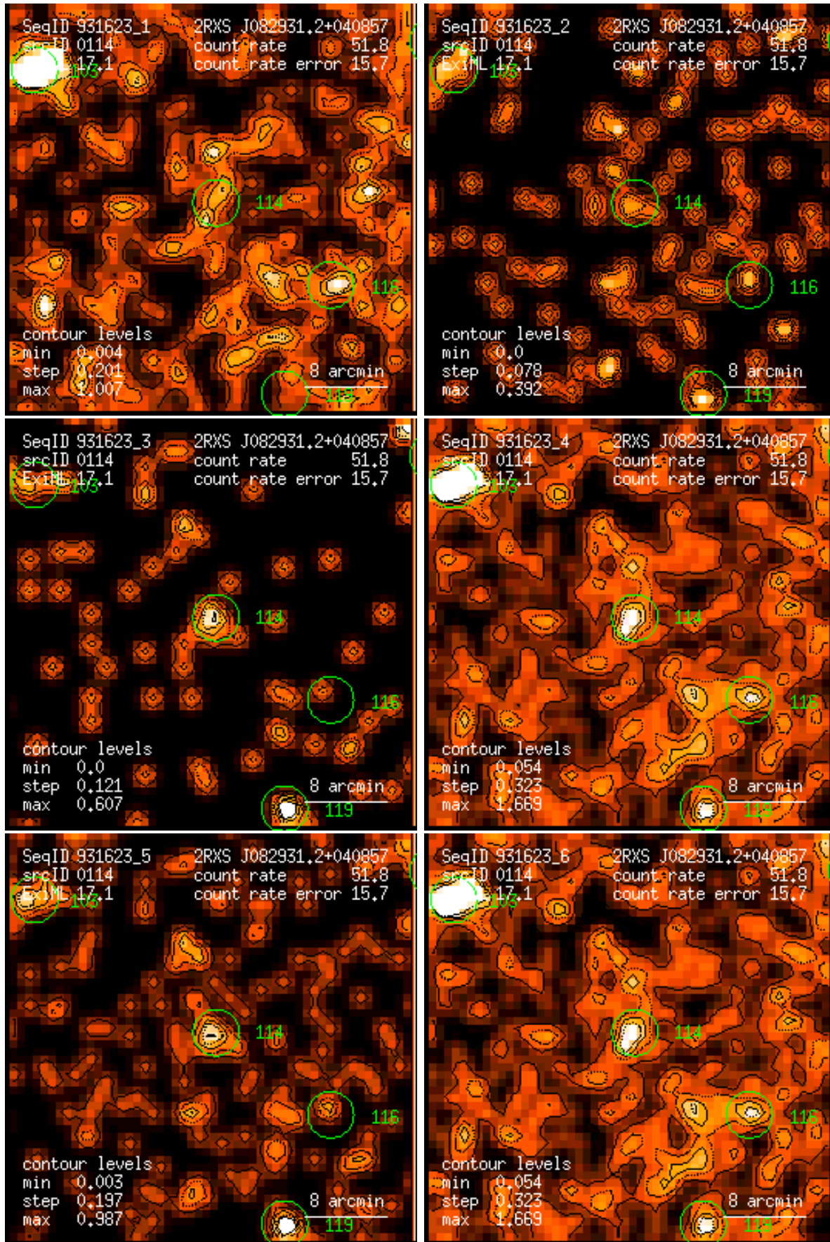
Figure 114: RASS 931623: detection 0114: band rate images, Gaussian filter: (1) PSPC channels 11 – 41, (2) 52 – 90, (3) 91 – 201, (4) 11 – 235, (5) 52 – 201, (6) 11 – 201. Broad band rates in counts/ks. Band rate contour levels in counts/ks/arcmin 2 .
