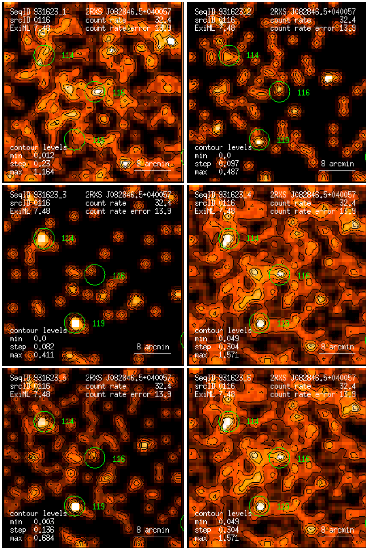
Figure 116: RASS 931623: detection 0116: band rate images, Gaussian filter: (1) PSPC channels 11 – 41, (2) 52 – 90, (3) 91 – 201, (4) 11 – 235, (5) 52 – 201, (6) 11 – 201. Broad band rates in counts/ks. Band rate contour levels in counts/ks/arcmin 2 .
