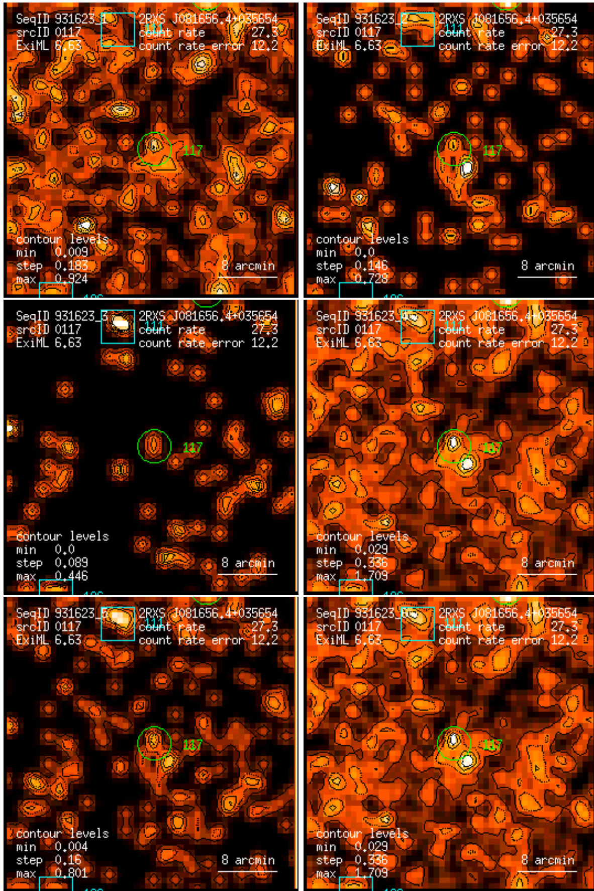
Figure 117: RASS 931623: detection 0117: band rate images, Gaussian filter: (1) PSPC channels 11 – 41, (2) 52 – 90, (3) 91 – 201, (4) 11 – 235, (5) 52 – 201, (6) 11 – 201. Broad band rates in counts/ks. Band rate contour levels in counts/ks/arcmin 2 .
