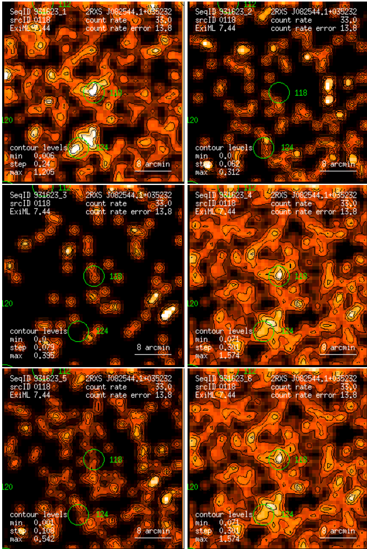
Figure 118: RASS 931623: detection 0118: band rate images, Gaussian filter: (1) PSPC channels 11 – 41, (2) 52 – 90, (3) 91 – 201, (4) 11 – 235, (5) 52 – 201, (6) 11 – 201. Broad band rates in counts/ks. Band rate contour levels in counts/ks/arcmin 2 .
