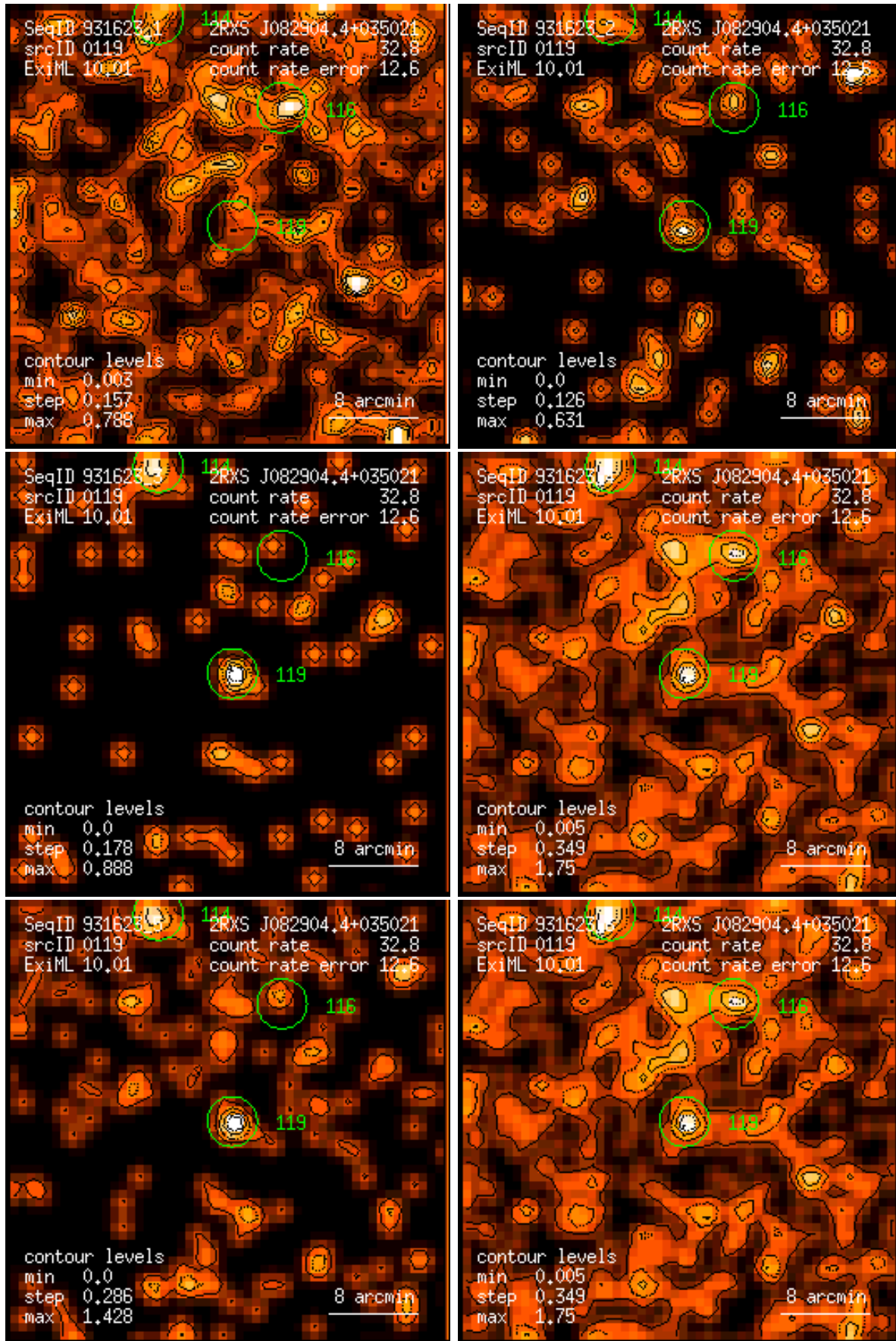
Figure 119: RASS 931623: detection 0119: band rate images, Gaussian filter: (1) PSPC channels 11 – 41, (2) 52 – 90, (3) 91 – 201, (4) 11 – 235, (5) 52 – 201, (6) 11 – 201. Broad band rates in counts/ks. Band rate contour levels in counts/ks/arcmin 2 .
