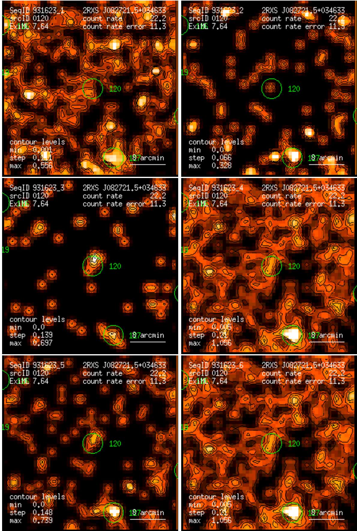
Figure 120: RASS 931623: detection 0120: band rate images, Gaussian filter: (1) PSPC channels 11 – 41, (2) 52 – 90, (3) 91 – 201, (4) 11 – 235, (5) 52 – 201, (6) 11 – 201. Broad band rates in counts/ks. Band rate contour levels in counts/ks/arcmin 2 .
