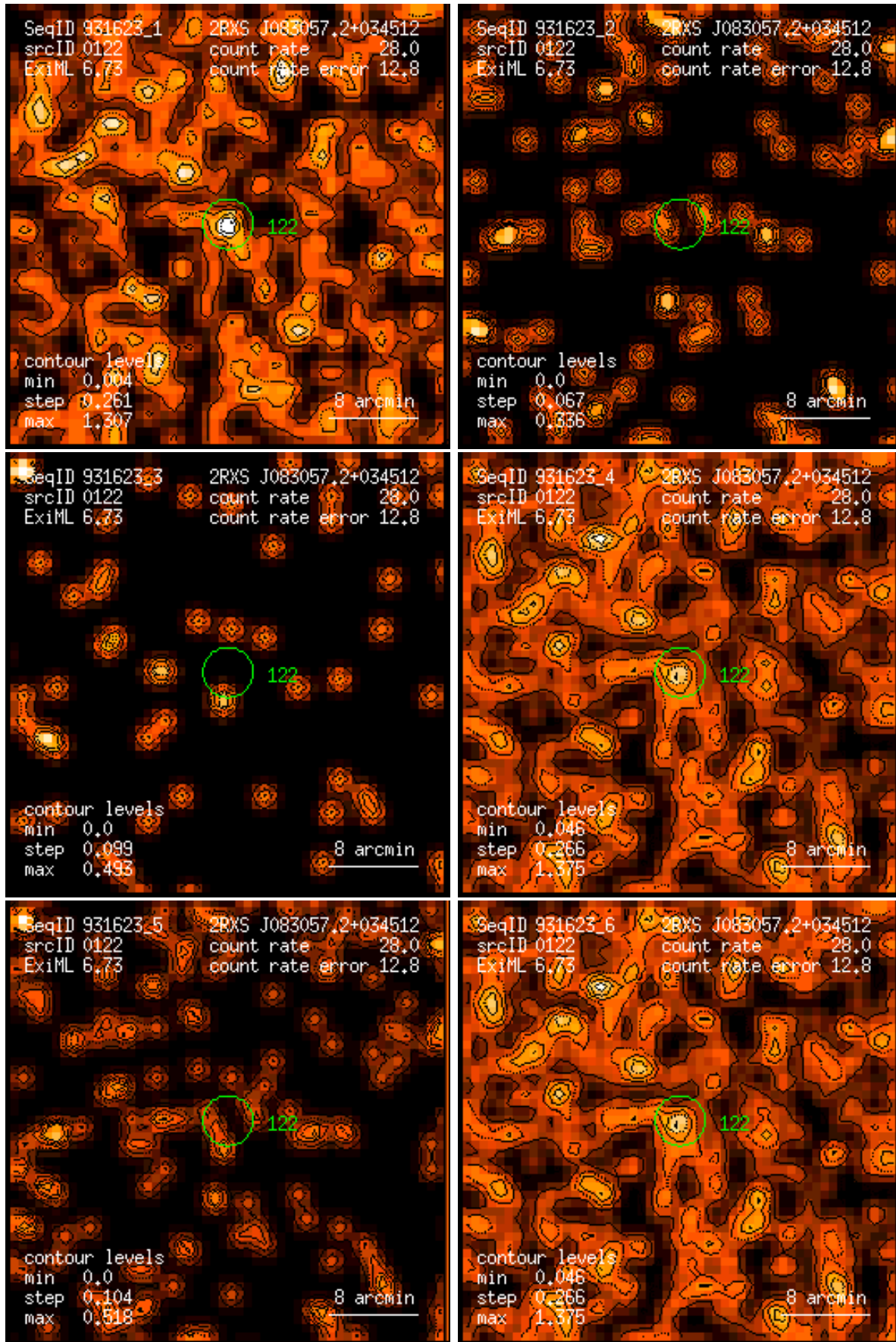
Figure 122: RASS 931623: detection 0122: band rate images, Gaussian filter: (1) PSPC channels 11 – 41, (2) 52 – 90, (3) 91 – 201, (4) 11 – 235, (5) 52 – 201, (6) 11 – 201. Broad band rates in counts/ks. Band rate contour levels in counts/ks/arcmin 2 .
