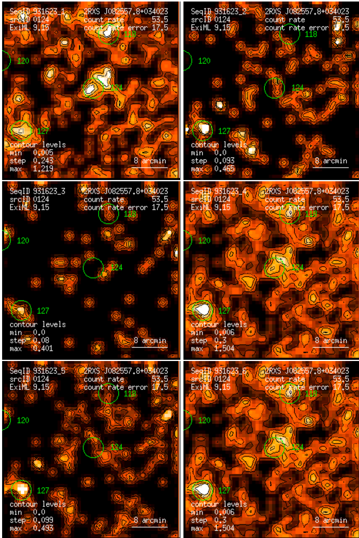
Figure 124: RASS 931623: detection 0124: band rate images, Gaussian filter: (1) PSPC channels 11 – 41, (2) 52 – 90, (3) 91 – 201, (4) 11 – 235, (5) 52 – 201, (6) 11 – 201. Broad band rates in counts/ks. Band rate contour levels in counts/ks/arcmin 2 .
