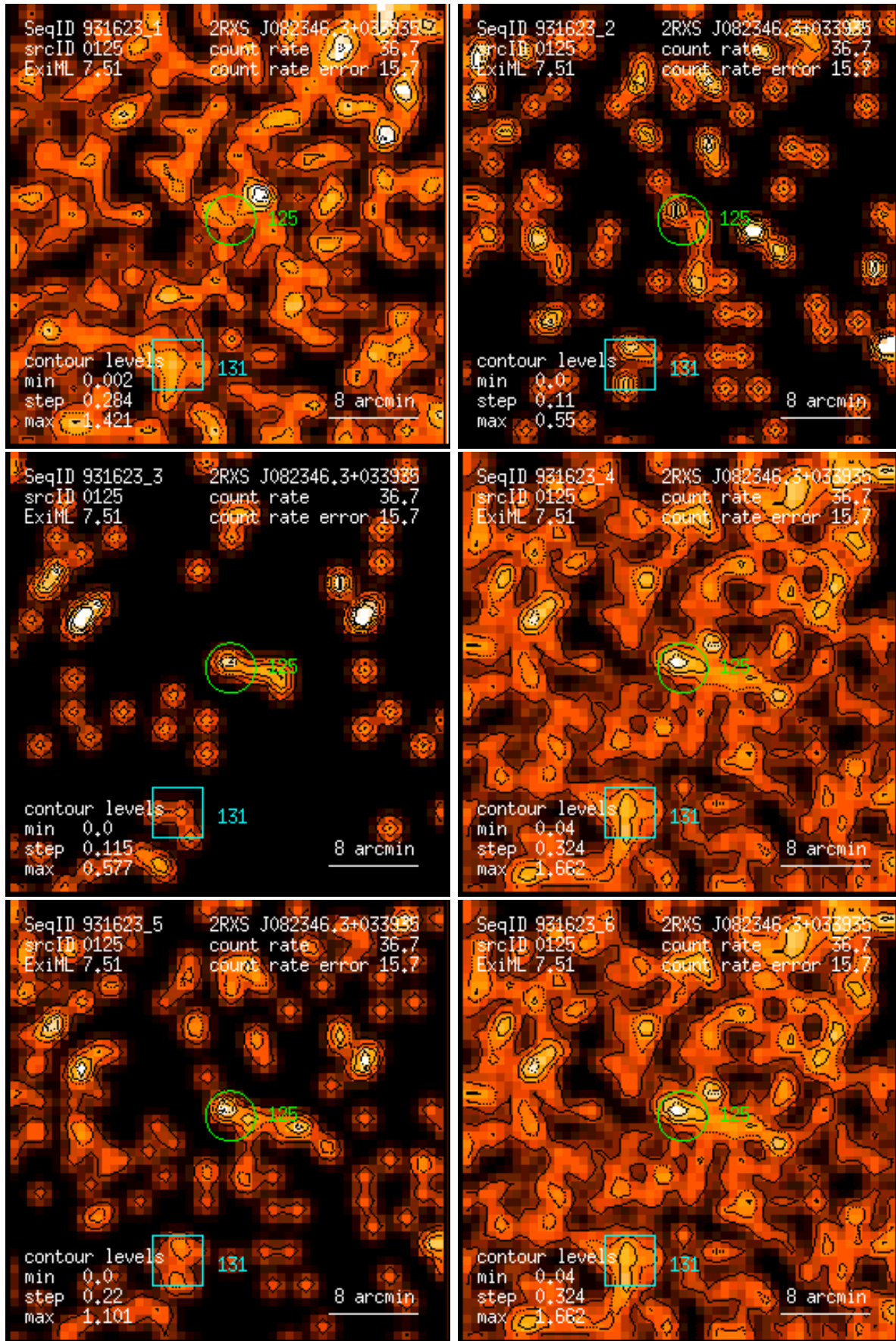
Figure 125: RASS 931623: detection 0125: band rate images, Gaussian filter: (1) PSPC channels 11 – 41, (2) 52 – 90, (3) 91 – 201, (4) 11 – 235, (5) 52 – 201, (6) 11 – 201. Broad band rates in counts/ks. Band rate contour levels in counts/ks/arcmin 2 .
