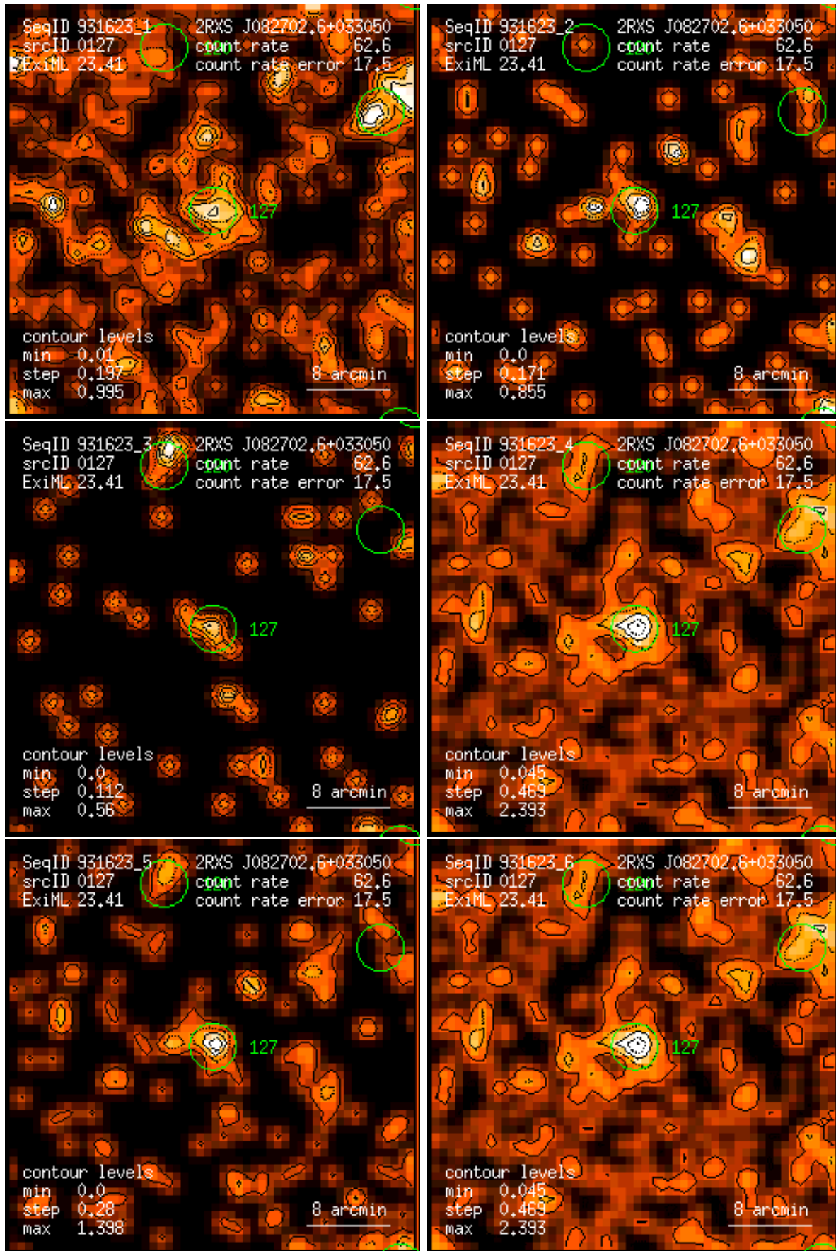
Figure 127: RASS 931623: detection 0127: band rate images, Gaussian filter: (1) PSPC channels 11 – 41, (2) 52 – 90, (3) 91 – 201, (4) 11 – 235, (5) 52 – 201, (6) 11 – 201. Broad band rates in counts/ks. Band rate contour levels in counts/ks/arcmin 2 .
