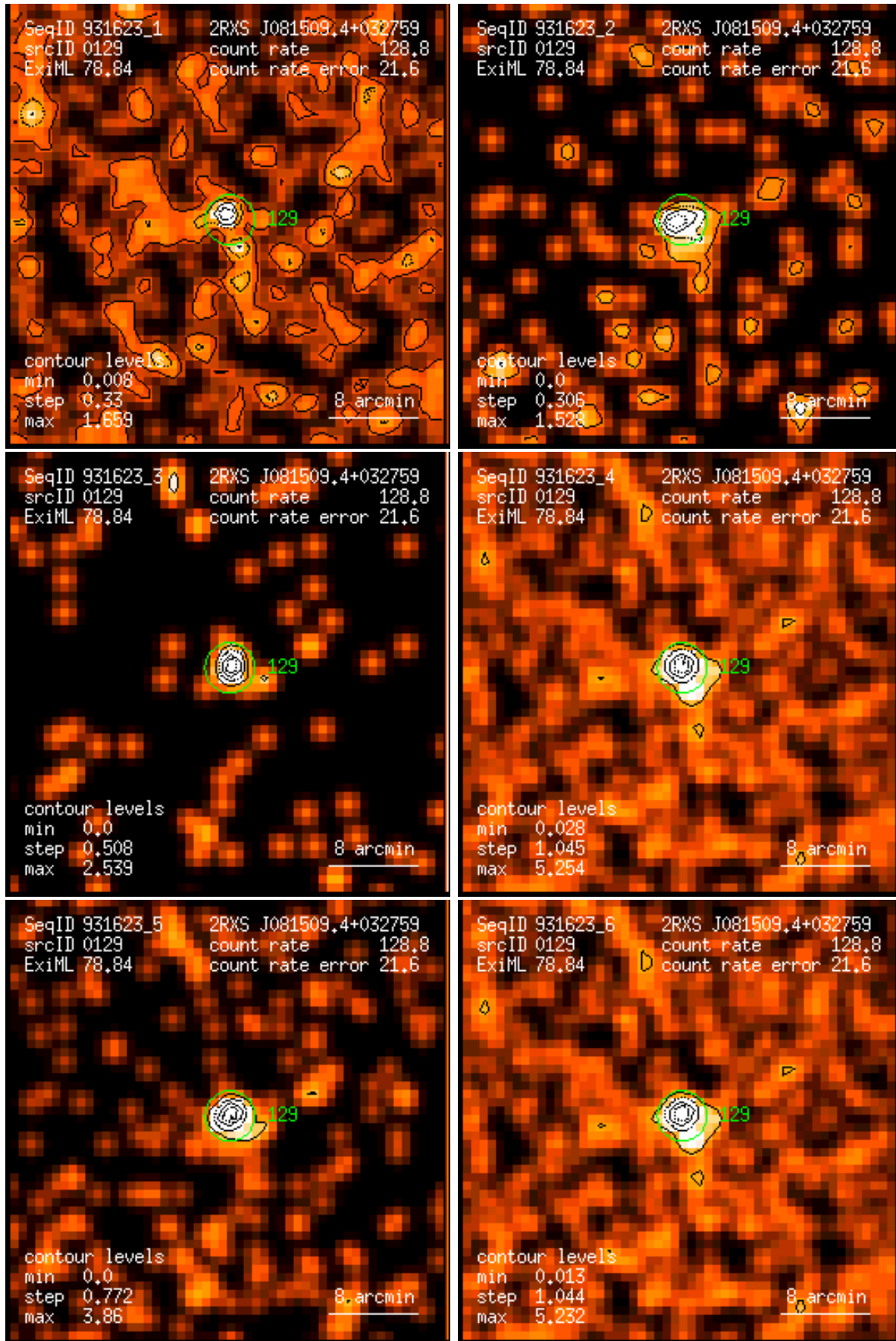
Figure 129: RASS 931623: detection 0129: band rate images, Gaussian filter: (1) PSPC channels 11 – 41, (2) 52 – 90, (3) 91 – 201, (4) 11 – 235, (5) 52 – 201, (6) 11 – 201. Broad band rates in counts/ks. Band rate contour levels in counts/ks/arcmin 2 .
