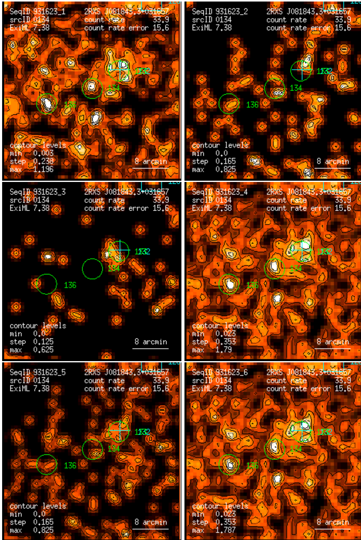
Figure 134: RASS 931623: detection 0134: band rate images, Gaussian filter: (1) PSPC channels 11 – 41, (2) 52 – 90, (3) 91 – 201, (4) 11 – 235, (5) 52 – 201, (6) 11 – 201. Broad band rates in counts/ks. Band rate contour levels in counts/ks/arcmin 2 .
