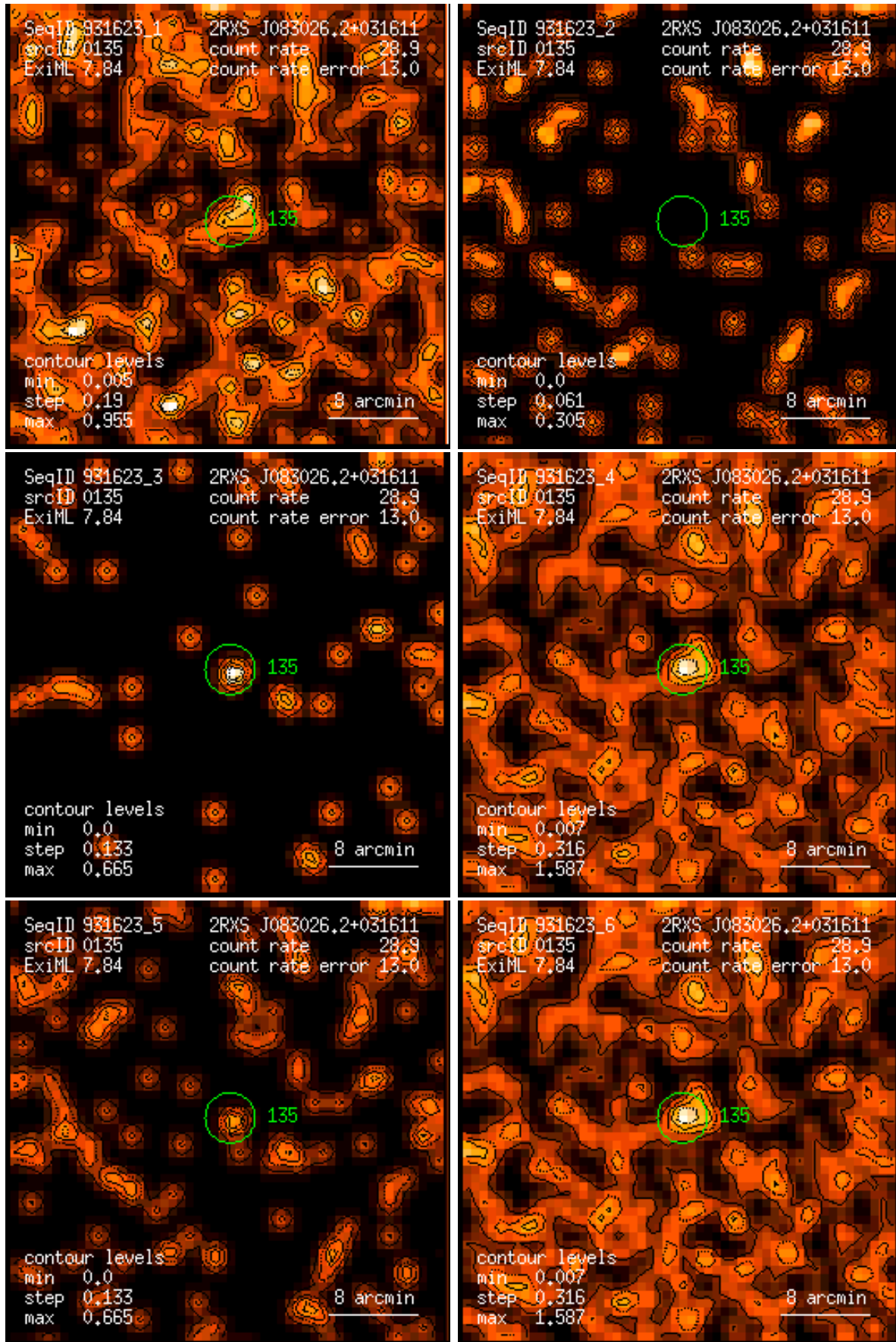
Figure 135: RASS 931623: detection 0135: band rate images, Gaussian filter: (1) PSPC channels 11 – 41, (2) 52 – 90, (3) 91 – 201, (4) 11 – 235, (5) 52 – 201, (6) 11 – 201. Broad band rates in counts/ks. Band rate contour levels in counts/ks/arcmin 2 .
