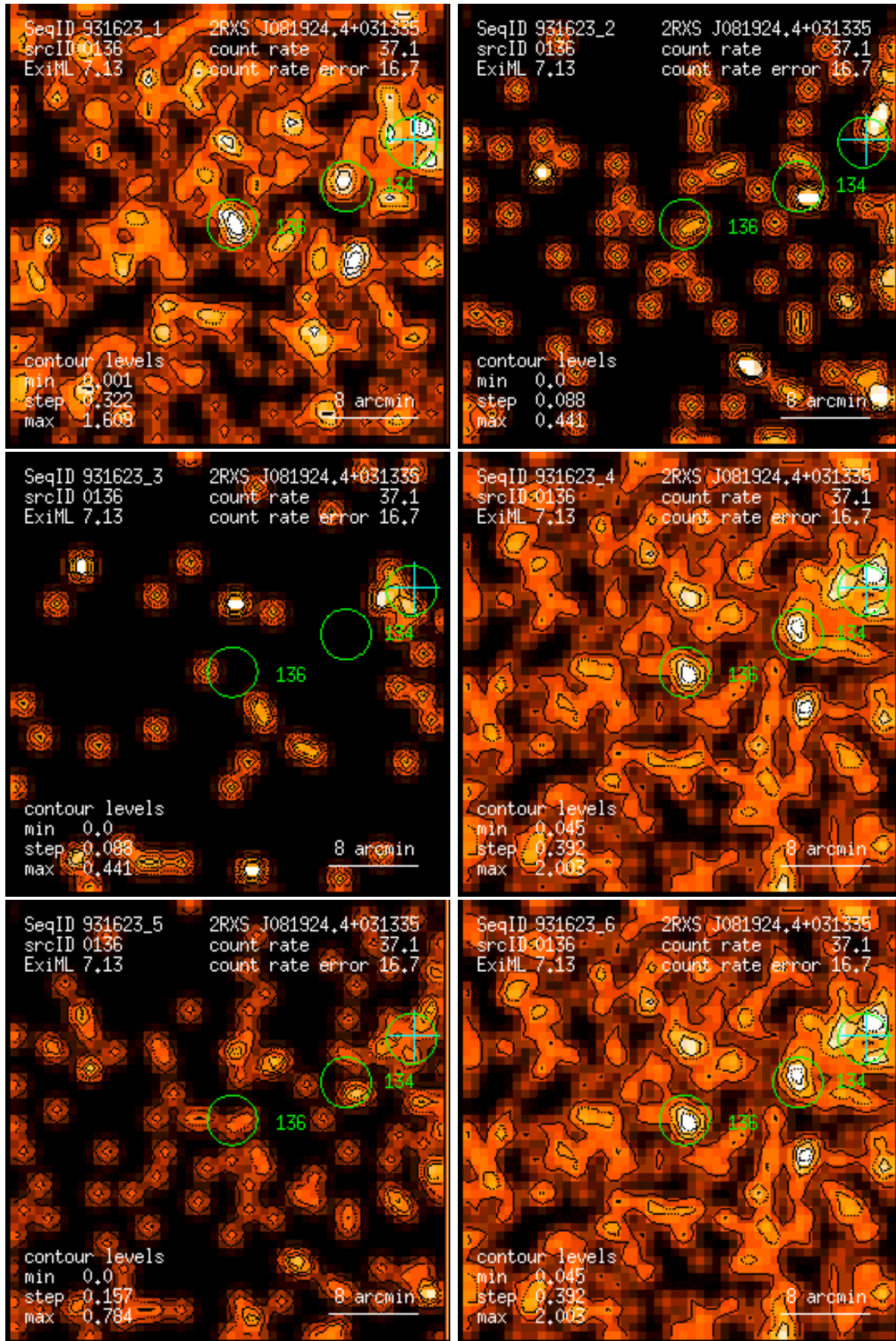
Figure 136: RASS 931623: detection 0136: band rate images, Gaussian filter: (1) PSPC channels 11 – 41, (2) 52 – 90, (3) 91 – 201, (4) 11 – 235, (5) 52 – 201, (6) 11 – 201. Broad band rates in counts/ks. Band rate contour levels in counts/ks/arcmin 2 .
