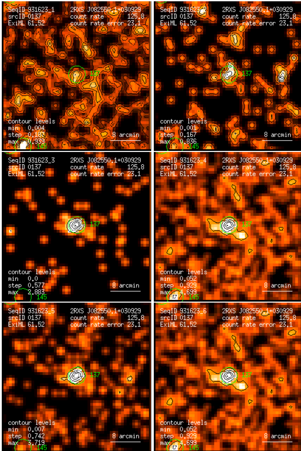
Figure 137: RASS 931623: detection 0137: band rate images, Gaussian filter: (1) PSPC channels 11 – 41, (2) 52 – 90, (3) 91 – 201, (4) 11 – 235, (5) 52 – 201, (6) 11 – 201. Broad band rates in counts/ks. Band rate contour levels in counts/ks/arcmin 2 .
