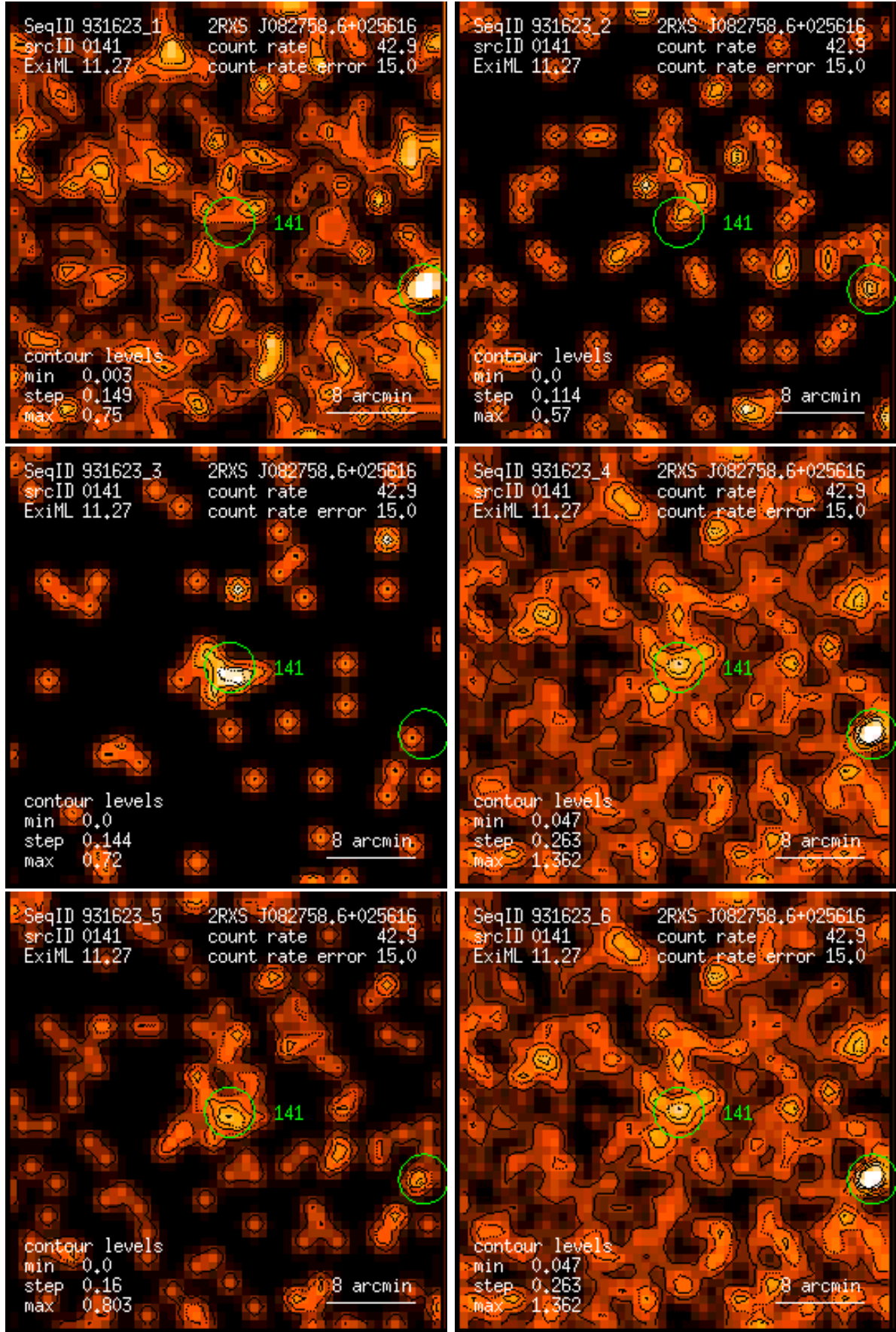
Figure 141: RASS 931623: detection 0141: band rate images, Gaussian filter: (1) PSPC channels 11 – 41, (2) 52 – 90, (3) 91 – 201, (4) 11 – 235, (5) 52 – 201, (6) 11 – 201. Broad band rates in counts/ks. Band rate contour levels in counts/ks/arcmin 2 .
