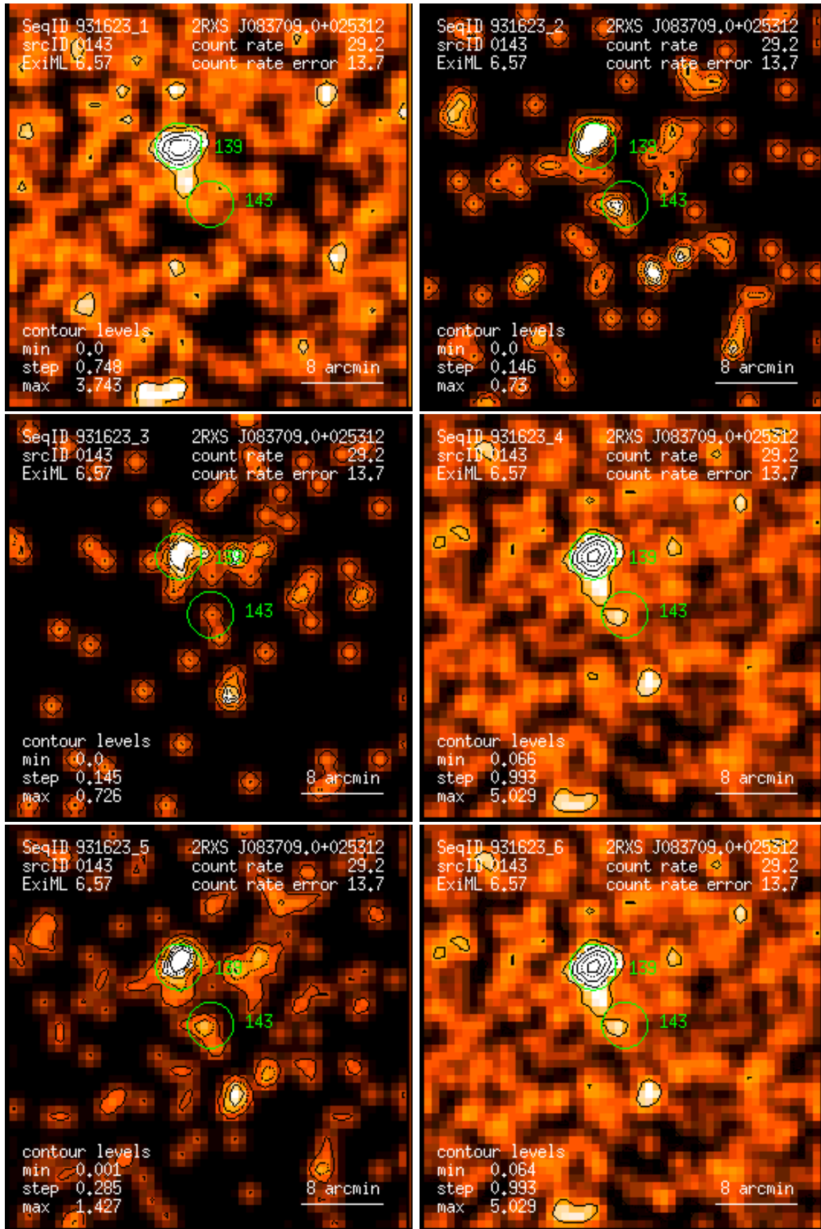
Figure 143: RASS 931623: detection 0143: band rate images, Gaussian filter: (1) PSPC channels 11 – 41, (2) 52 – 90, (3) 91 – 201, (4) 11 – 235, (5) 52 – 201, (6) 11 – 201. Broad band rates in counts/ks. Band rate contour levels in counts/ks/arcmin 2 .
