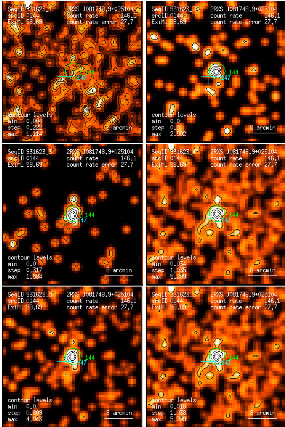
Figure 144: RASS 931623: detection 0144: band rate images, Gaussian filter: (1) PSPC channels 11 – 41, (2) 52 – 90, (3) 91 – 201, (4) 11 – 235, (5) 52 – 201, (6) 11 – 201. Broad band rates in counts/ks. Band rate contour levels in counts/ks/arcmin 2 .
