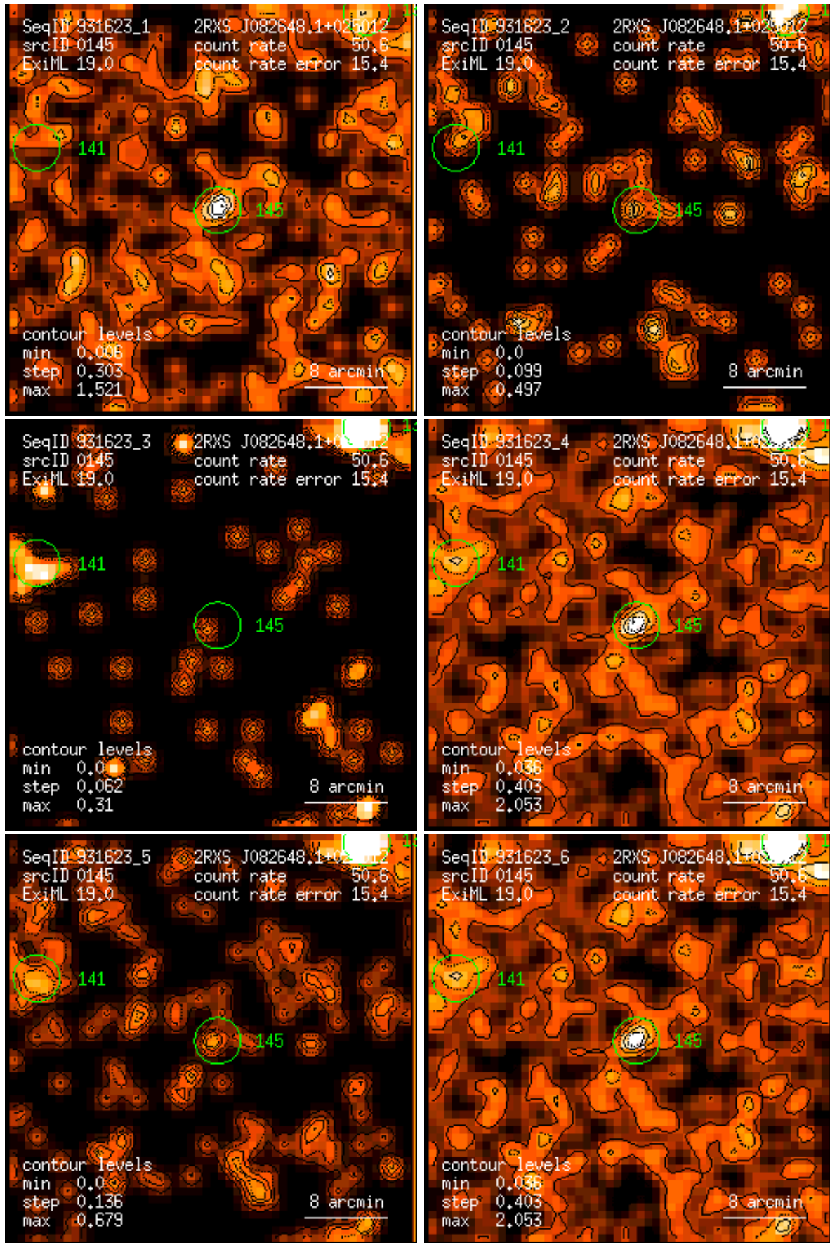
Figure 145: RASS 931623: detection 0145: band rate images, Gaussian filter: (1) PSPC channels 11 – 41, (2) 52 – 90, (3) 91 – 201, (4) 11 – 235, (5) 52 – 201, (6) 11 – 201. Broad band rates in counts/ks. Band rate contour levels in counts/ks/arcmin 2 .
