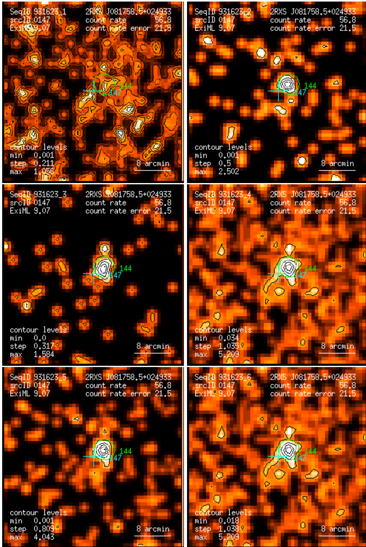
Figure 147: RASS 931623: detection 0147: band rate images, Gaussian filter: (1) PSPC channels 11 – 41, (2) 52 – 90, (3) 91 – 201, (4) 11 – 235, (5) 52 – 201, (6) 11 – 201. Broad band rates in counts/ks. Band rate contour levels in counts/ks/arcmin 2 .
