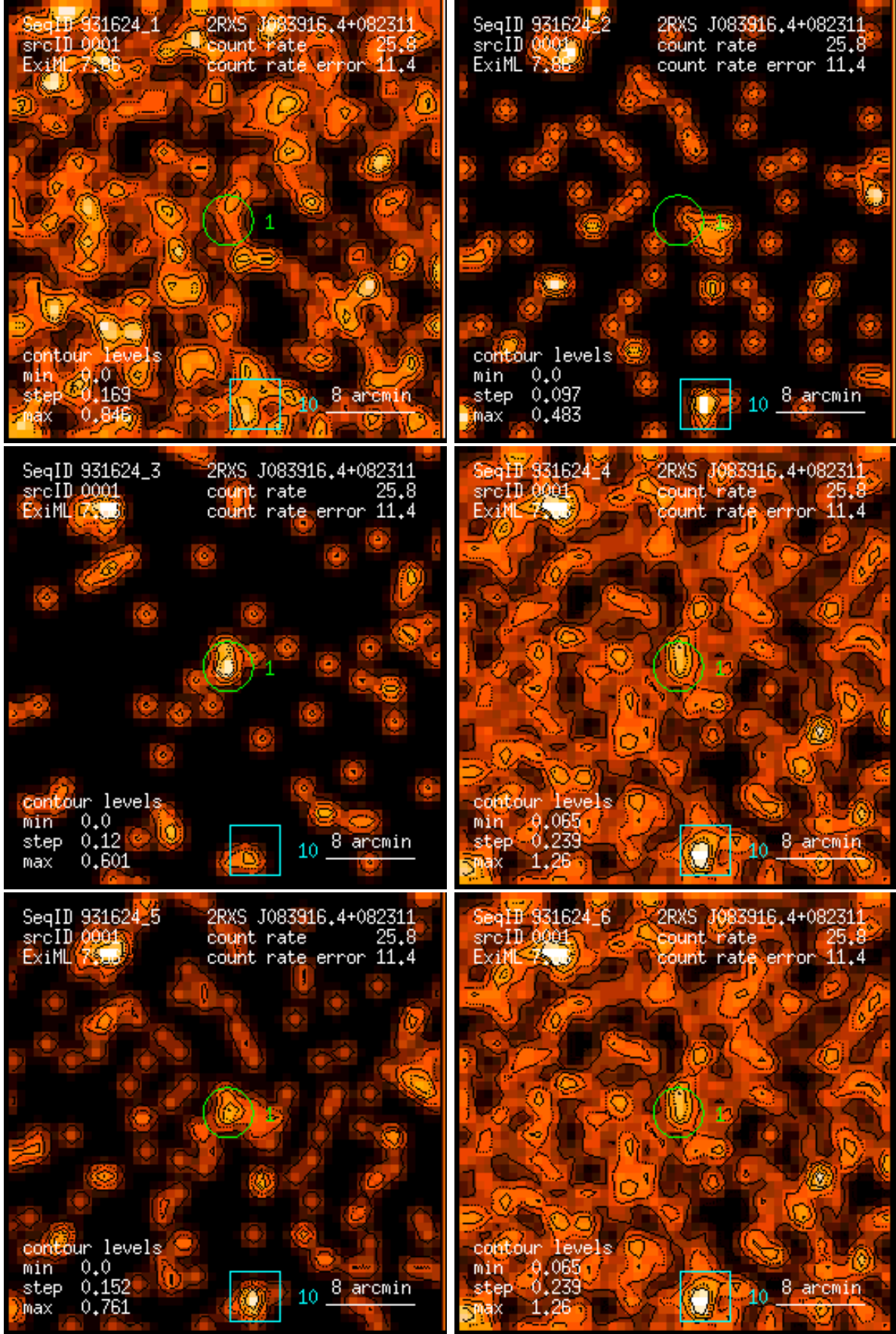
Figure 1: RASS 931624: detection 0001: band rate images, Gaussian filter: (1) PSPC channels 11 – 41, (2) 52 – 90, (3) 91 – 201, (4) 11 – 235, (5) 52 – 201, (6) 11 – 201. Broad band rates in counts/ks. Band rate contour levels in counts/ks/arcmin 2 .
