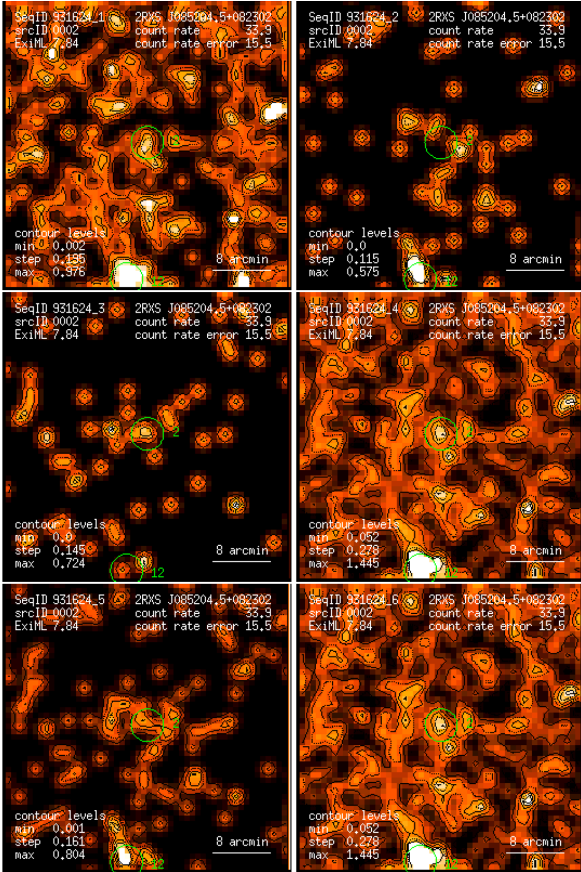
Figure 2: RASS 931624: detection 0002: band rate images, Gaussian filter: (1) PSPC channels 11 – 41, (2) 52 – 90, (3) 91 – 201, (4) 11 – 235, (5) 52 – 201, (6) 11 – 201. Broad band rates in counts/ks. Band rate contour levels in counts/ks/arcmin 2 .
