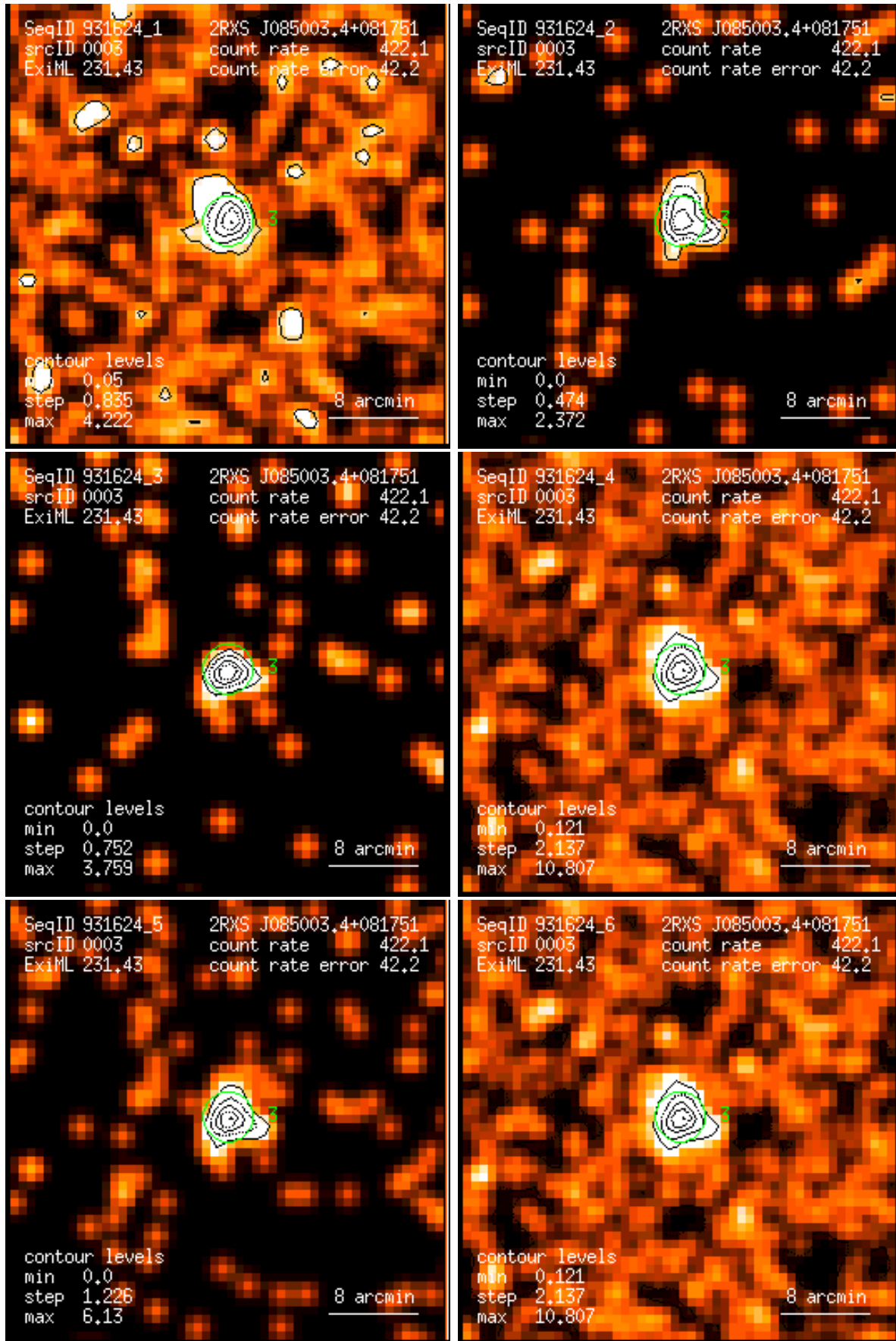
Figure 3: RASS 931624: detection 0003: band rate images, Gaussian filter: (1) PSPC channels 11 – 41, (2) 52 – 90, (3) 91 – 201, (4) 11 – 235, (5) 52 – 201, (6) 11 – 201. Broad band rates in counts/ks. Band rate contour levels in counts/ks/arcmin 2 .
