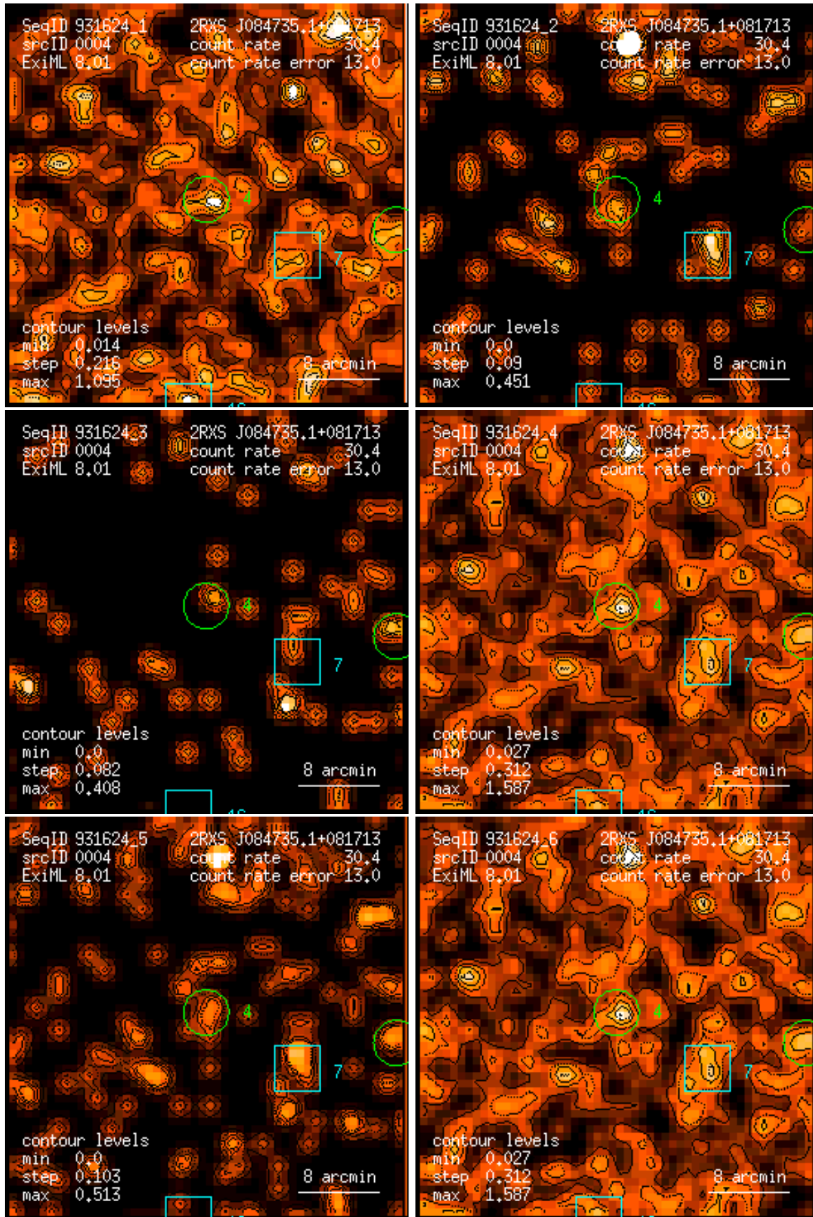
Figure 4: RASS 931624: detection 0004: band rate images, Gaussian filter: (1) PSPC channels 11 – 41, (2) 52 – 90, (3) 91 – 201, (4) 11 – 235, (5) 52 – 201, (6) 11 – 201. Broad band rates in counts/ks. Band rate contour levels in counts/ks/arcmin 2 .
