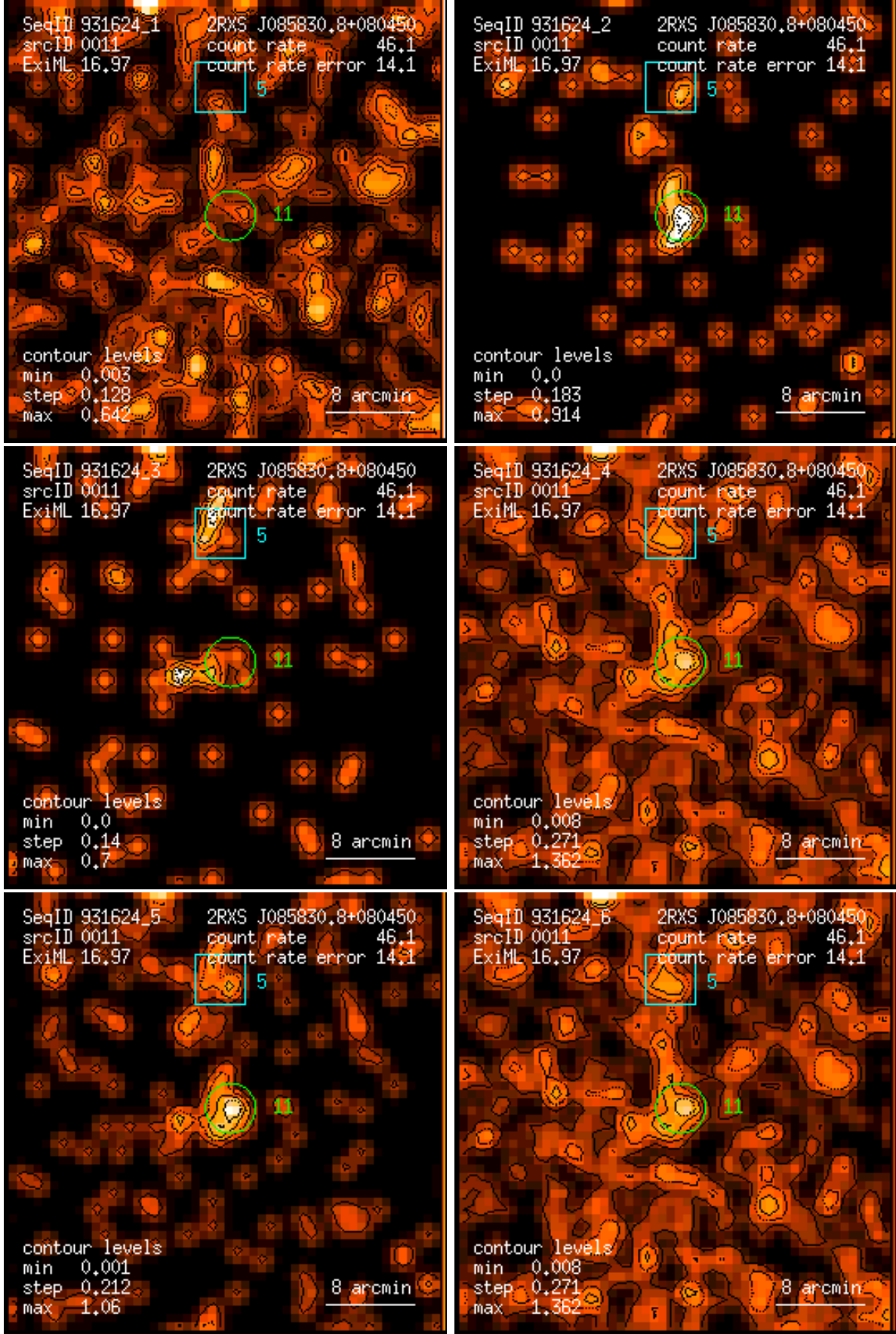
Figure 11: RASS 931624: detection 0011: band rate images, Gaussian filter: (1) PSPC channels 11 – 41, (2) 52 – 90, (3) 91 – 201, (4) 11 – 235, (5) 52 – 201, (6) 11 – 201. Broad band rates in counts/ks. Band rate contour levels in counts/ks/arcmin 2 .
